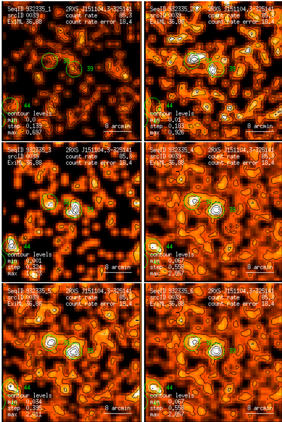
Figure 39: RASS 932335: detection 0039: band rate images, Gaussian filter: (1) PSPC channels 11 – 41, (2) 52 – 90, (3) 91 – 201, (4) 11 – 235, (5) 52 – 201, (6) 11 – 201. Broad band rates in counts/ks. Band rate contour levels in counts/ks/arcmin 2 .
