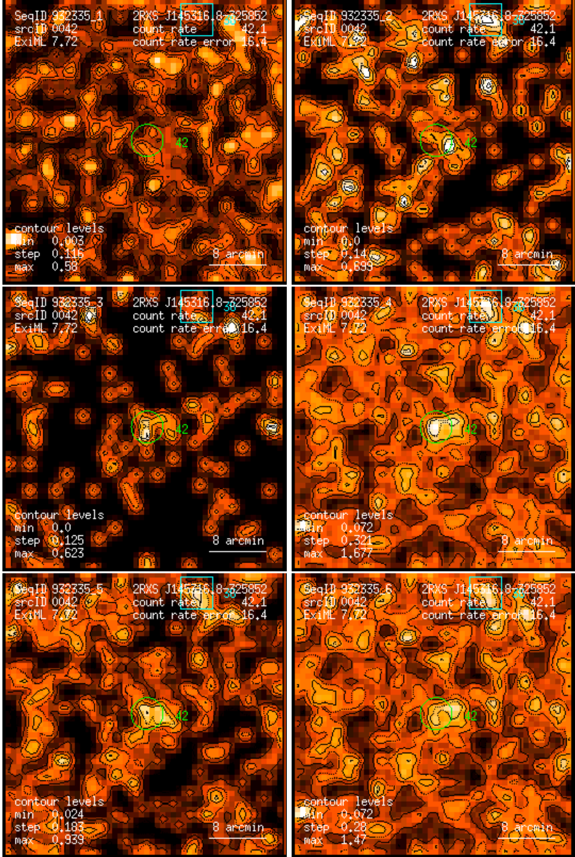
Figure 42: RASS 932335: detection 0042: band rate images, Gaussian filter: (1) PSPC channels 11 – 41, (2) 52 – 90, (3) 91 – 201, (4) 11 – 235, (5) 52 – 201, (6) 11 – 201. Broad band rates in counts/ks. Band rate contour levels in counts/ks/arcmin 2 .
