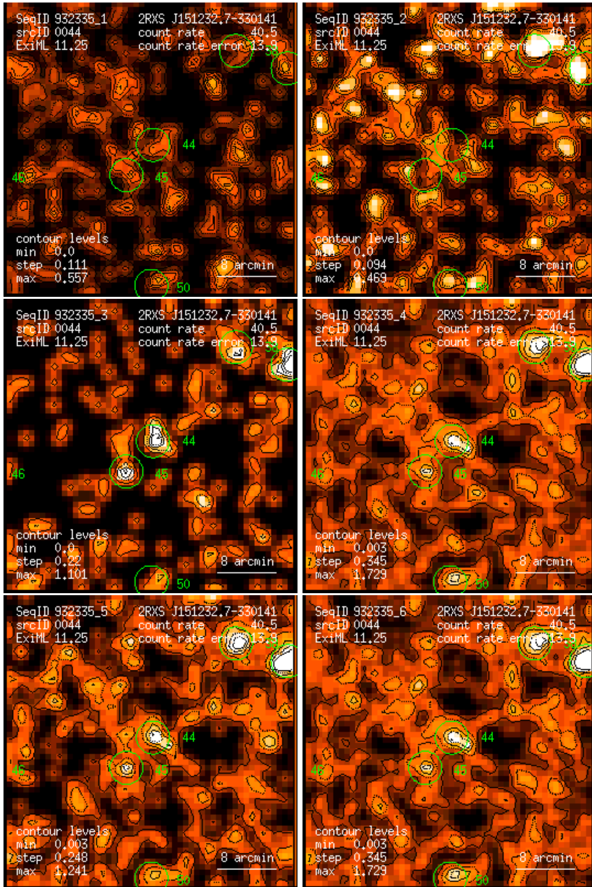
Figure 44: RASS 932335: detection 0044: band rate images, Gaussian filter: (1) PSPC channels 11 – 41, (2) 52 – 90, (3) 91 – 201, (4) 11 – 235, (5) 52 – 201, (6) 11 – 201. Broad band rates in counts/ks. Band rate contour levels in counts/ks/arcmin 2 .
