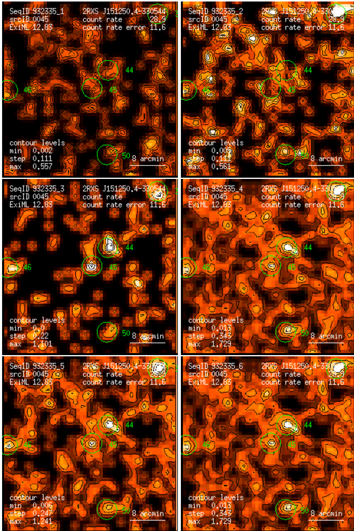
Figure 45: RASS 932335: detection 0045: band rate images, Gaussian filter: (1) PSPC channels 11 – 41, (2) 52 – 90, (3) 91 – 201, (4) 11 – 235, (5) 52 – 201, (6) 11 – 201. Broad band rates in counts/ks. Band rate contour levels in counts/ks/arcmin 2 .
