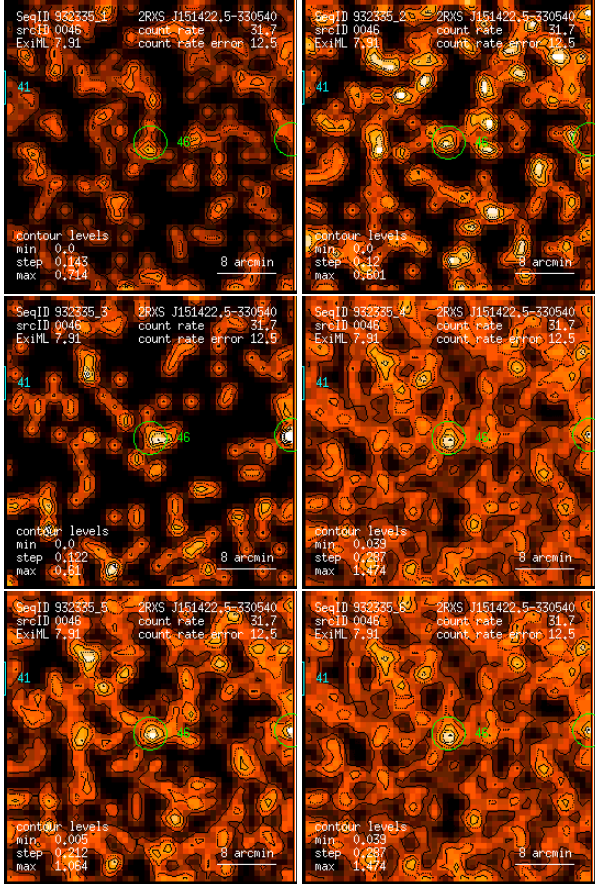
Figure 46: RASS 932335: detection 0046: band rate images, Gaussian filter: (1) PSPC channels 11 – 41, (2) 52 – 90, (3) 91 – 201, (4) 11 – 235, (5) 52 – 201, (6) 11 – 201. Broad band rates in counts/ks. Band rate contour levels in counts/ks/arcmin 2 .
