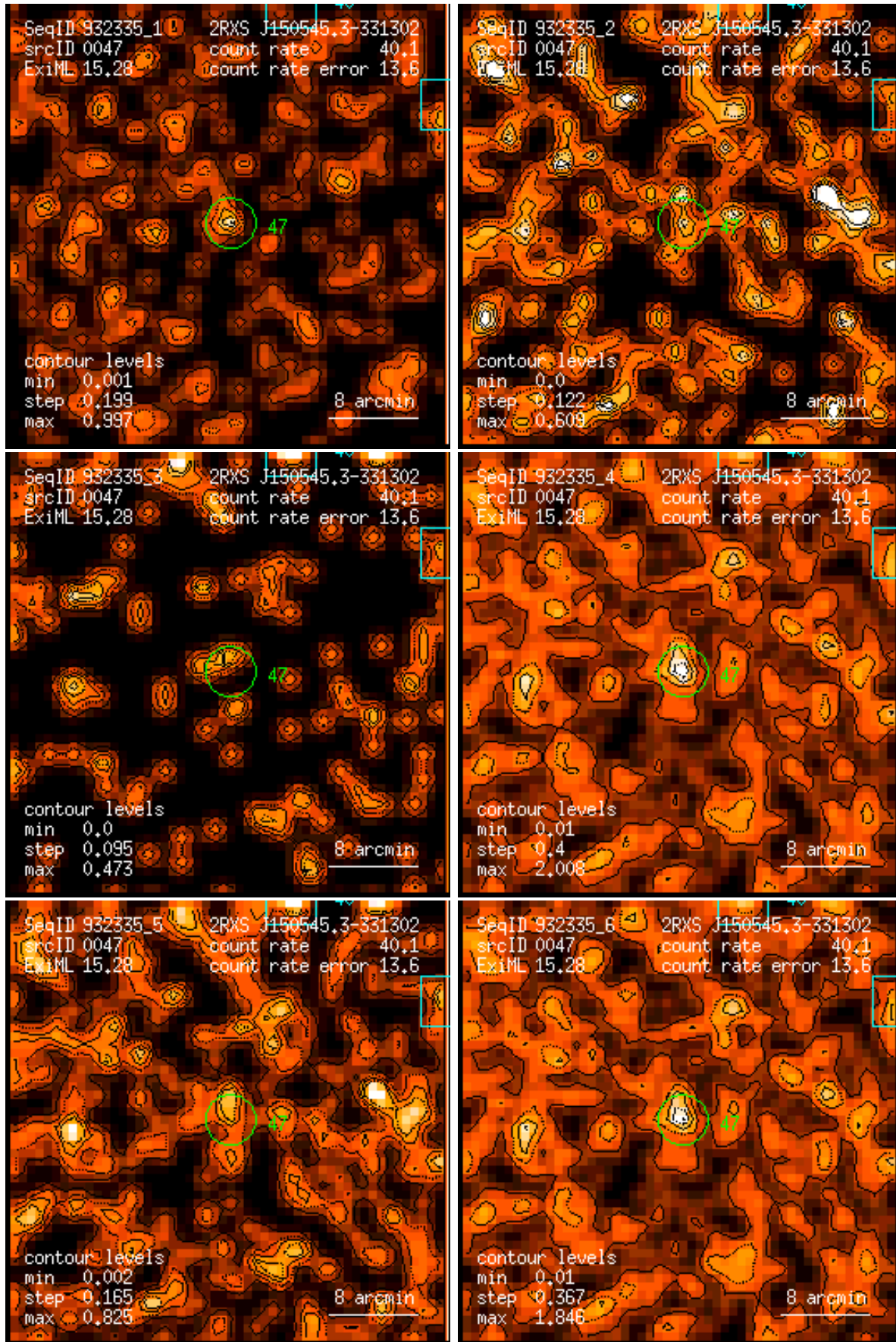
Figure 47: RASS 932335: detection 0047: band rate images, Gaussian filter: (1) PSPC channels 11 – 41, (2) 52 – 90, (3) 91 – 201, (4) 11 – 235, (5) 52 – 201, (6) 11 – 201. Broad band rates in counts/ks. Band rate contour levels in counts/ks/arcmin 2 .
