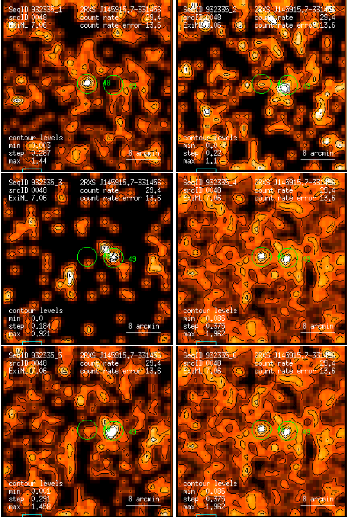
Figure 48: RASS 932335: detection 0048: band rate images, Gaussian filter: (1) PSPC channels 11 – 41, (2) 52 – 90, (3) 91 – 201, (4) 11 – 235, (5) 52 – 201, (6) 11 – 201. Broad band rates in counts/ks. Band rate contour levels in counts/ks/arcmin 2 .
