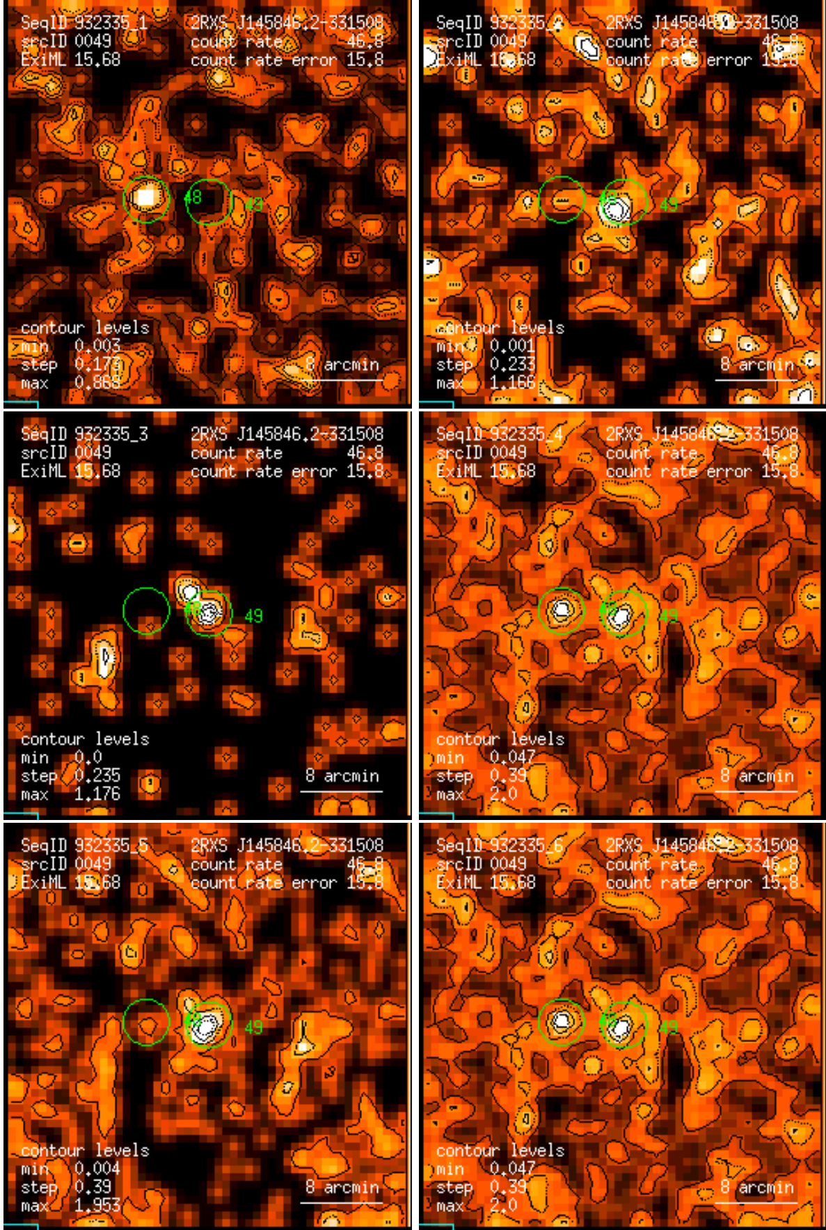
Figure 49: RASS 932335: detection 0049: band rate images, Gaussian filter: (1) PSPC channels 11 – 41, (2) 52 – 90, (3) 91 – 201, (4) 11 – 235, (5) 52 – 201, (6) 11 – 201. Broad band rates in counts/ks. Band rate contour levels in counts/ks/arcmin 2 .
