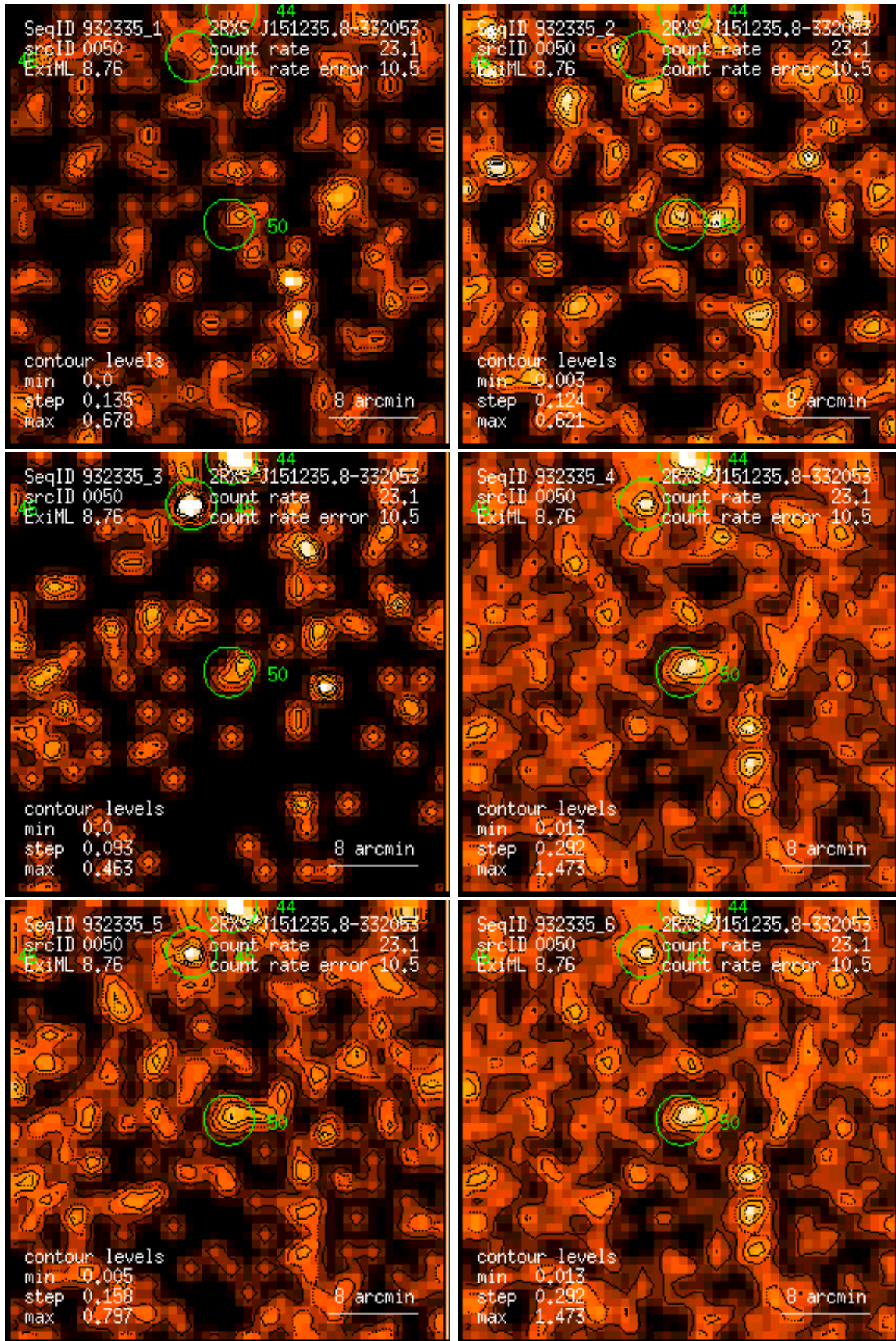
Figure 50: RASS 932335: detection 0050: band rate images, Gaussian filter: (1) PSPC channels 11 – 41, (2) 52 – 90, (3) 91 – 201, (4) 11 – 235, (5) 52 – 201, (6) 11 – 201. Broad band rates in counts/ks. Band rate contour levels in counts/ks/arcmin 2 .
