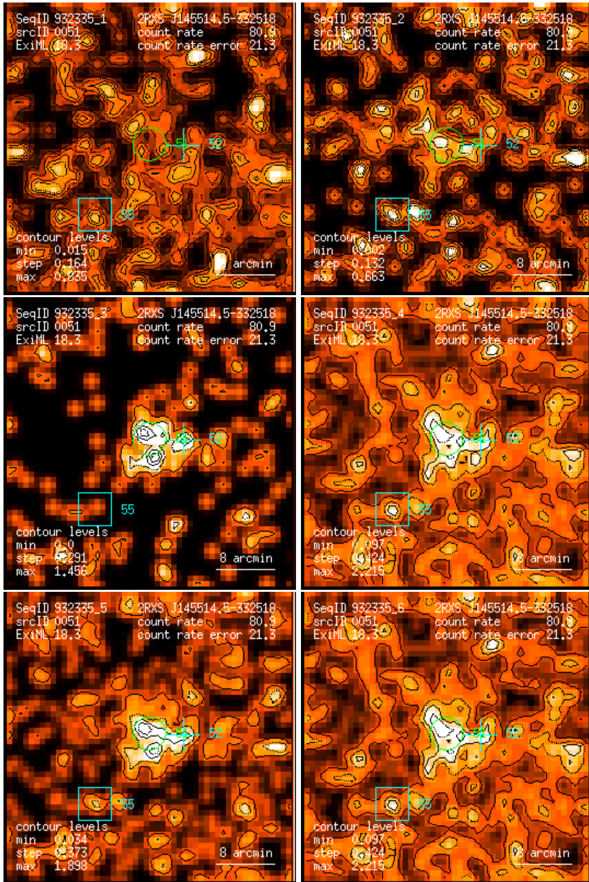
Figure 51: RASS 932335: detection 0051: band rate images, Gaussian filter: (1) PSPC channels 11 – 41, (2) 52 – 90, (3) 91 – 201, (4) 11 – 235, (5) 52 – 201, (6) 11 – 201. Broad band rates in counts/ks. Band rate contour levels in counts/ks/arcmin 2 .
