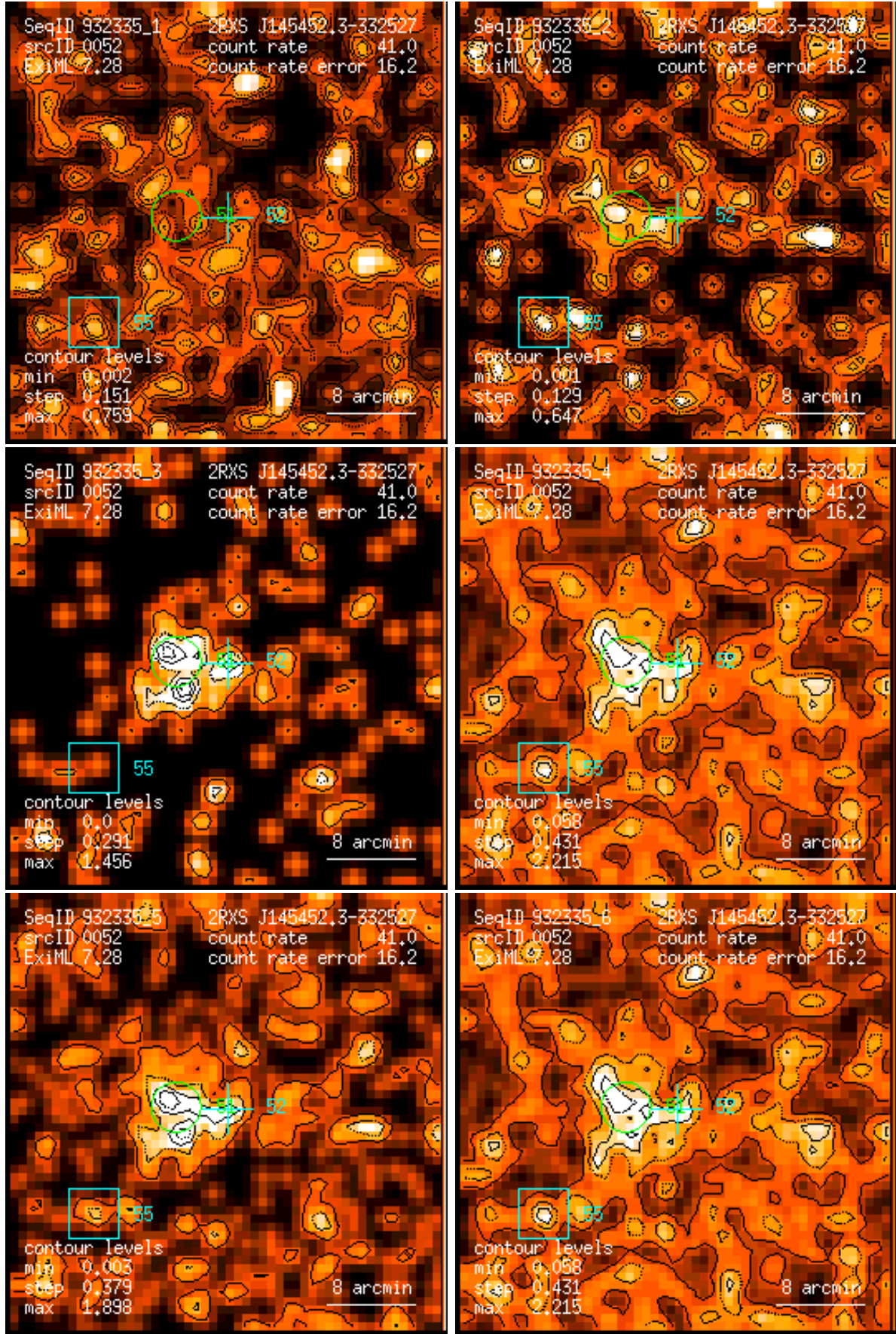
Figure 52: RASS 932335: detection 0052: band rate images, Gaussian filter: (1) PSPC channels 11 – 41, (2) 52 – 90, (3) 91 – 201, (4) 11 – 235, (5) 52 – 201, (6) 11 – 201. Broad band rates in counts/ks. Band rate contour levels in counts/ks/arcmin 2 .
