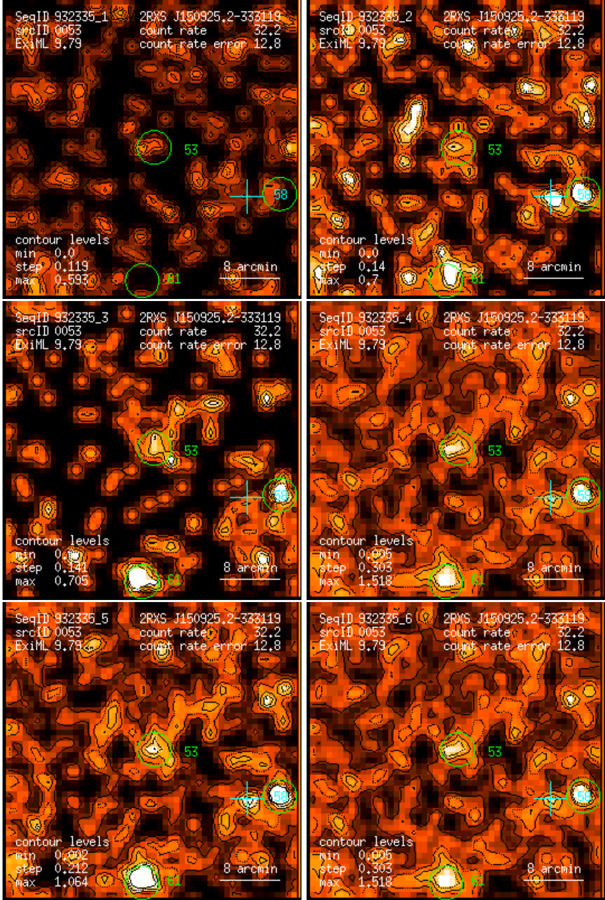
Figure 53: RASS 932335: detection 0053: band rate images, Gaussian filter: (1) PSPC channels 11 – 41, (2) 52 – 90, (3) 91 – 201, (4) 11 – 235, (5) 52 – 201, (6) 11 – 201. Broad band rates in counts/ks. Band rate contour levels in counts/ks/arcmin 2 .
