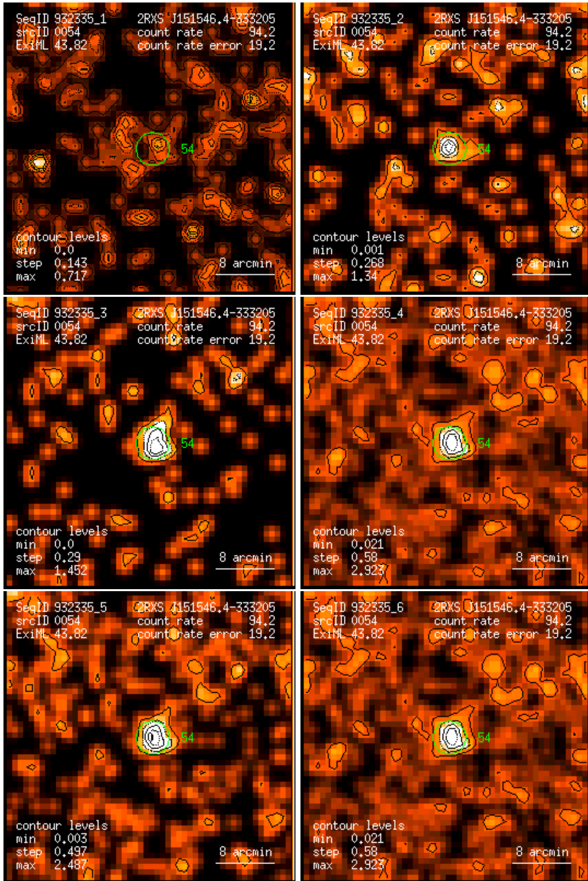
Figure 54: RASS 932335: detection 0054: band rate images, Gaussian filter: (1) PSPC channels 11 – 41, (2) 52 – 90, (3) 91 – 201, (4) 11 – 235, (5) 52 – 201, (6) 11 – 201. Broad band rates in counts/ks. Band rate contour levels in counts/ks/arcmin 2 .
