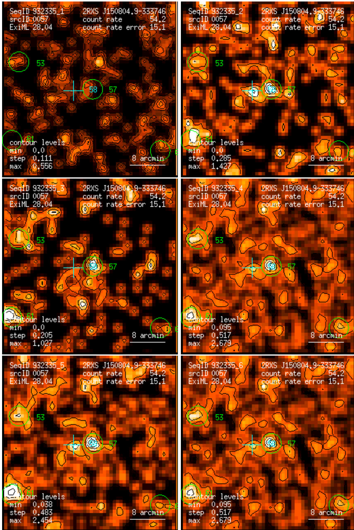
Figure 57: RASS 932335: detection 0057: band rate images, Gaussian filter: (1) PSPC channels 11 – 41, (2) 52 – 90, (3) 91 – 201, (4) 11 – 235, (5) 52 – 201, (6) 11 – 201. Broad band rates in counts/ks. Band rate contour levels in counts/ks/arcmin 2 .
