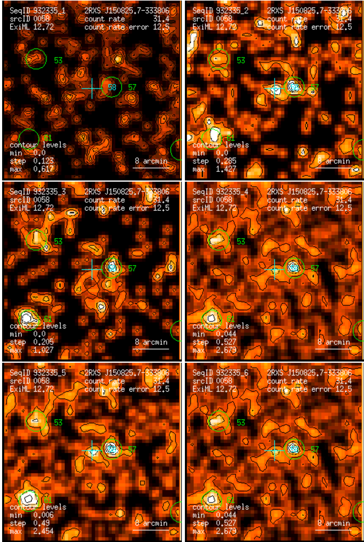
Figure 58: RASS 932335: detection 0058: band rate images, Gaussian filter: (1) PSPC channels 11 – 41, (2) 52 – 90, (3) 91 – 201, (4) 11 – 235, (5) 52 – 201, (6) 11 – 201. Broad band rates in counts/ks. Band rate contour levels in counts/ks/arcmin 2 .
