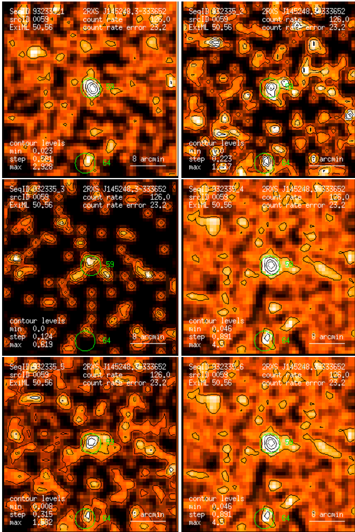
Figure 59: RASS 932335: detection 0059: band rate images, Gaussian filter: (1) PSPC channels 11 – 41, (2) 52 – 90, (3) 91 – 201, (4) 11 – 235, (5) 52 – 201, (6) 11 – 201. Broad band rates in counts/ks. Band rate contour levels in counts/ks/arcmin 2 .
