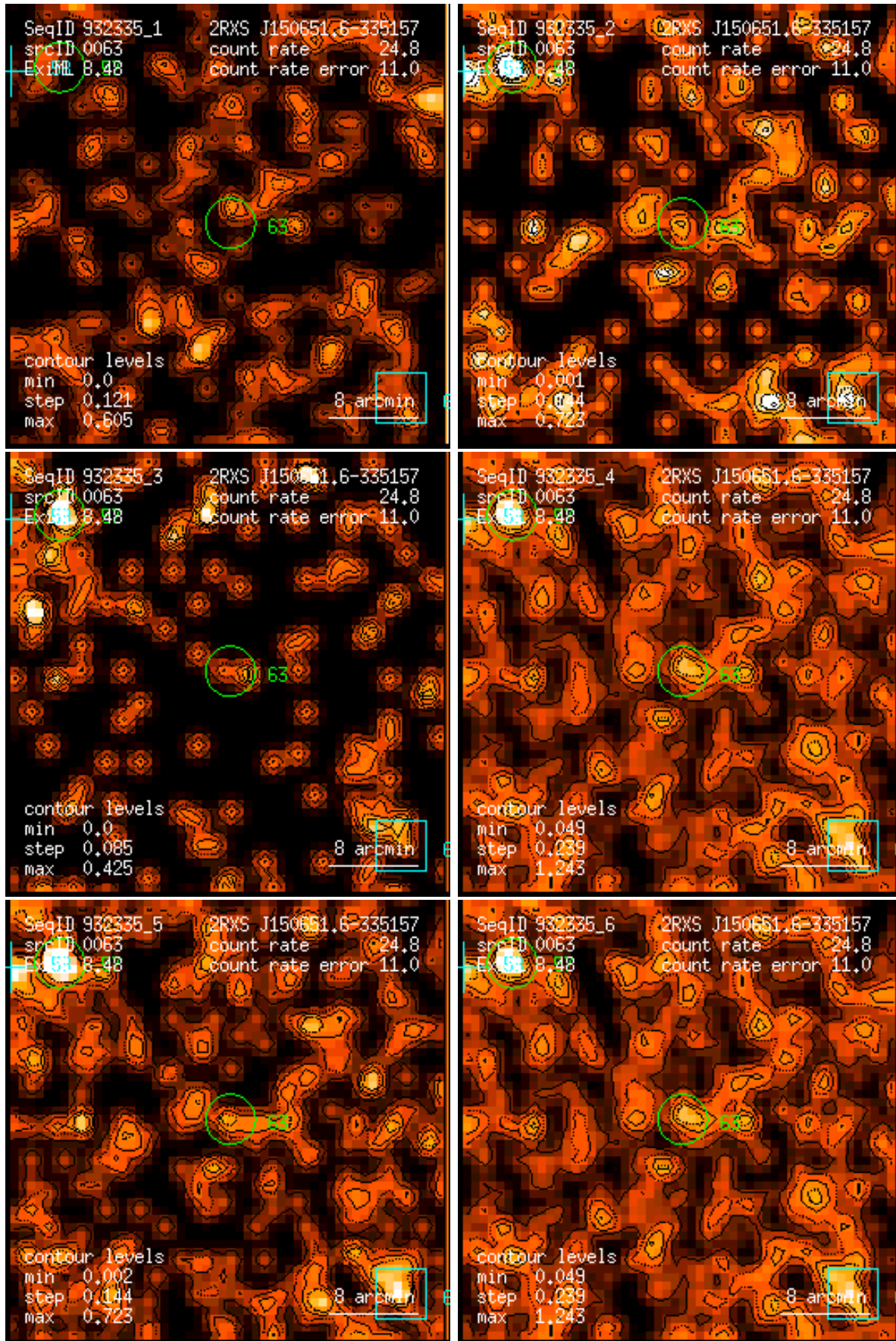
Figure 63: RASS 932335: detection 0063: band rate images, Gaussian filter: (1) PSPC channels 11 – 41, (2) 52 – 90, (3) 91 – 201, (4) 11 – 235, (5) 52 – 201, (6) 11 – 201. Broad band rates in counts/ks. Band rate contour levels in counts/ks/arcmin 2 .
