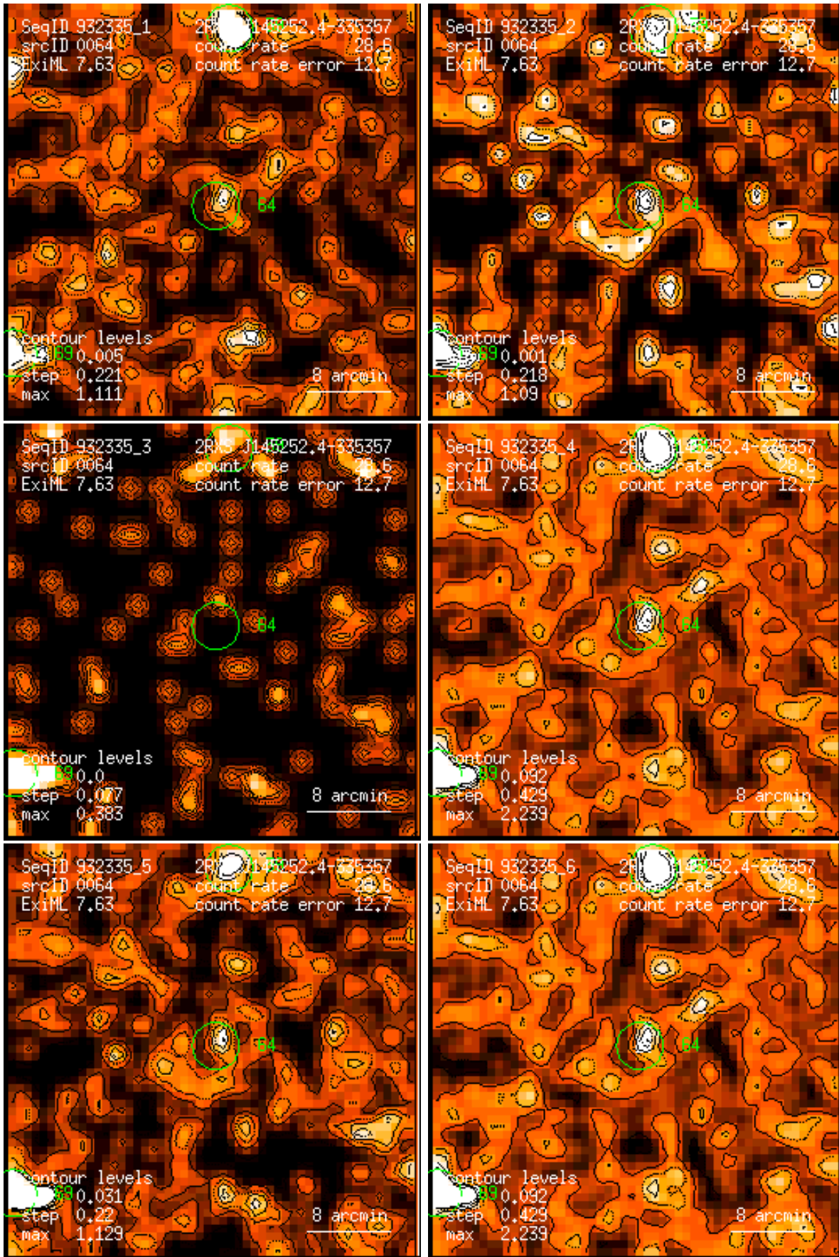
Figure 64: RASS 932335: detection 0064: band rate images, Gaussian filter: (1) PSPC channels 11 – 41, (2) 52 – 90, (3) 91 – 201, (4) 11 – 235, (5) 52 – 201, (6) 11 – 201. Broad band rates in counts/ks. Band rate contour levels in counts/ks/arcmin 2 .
