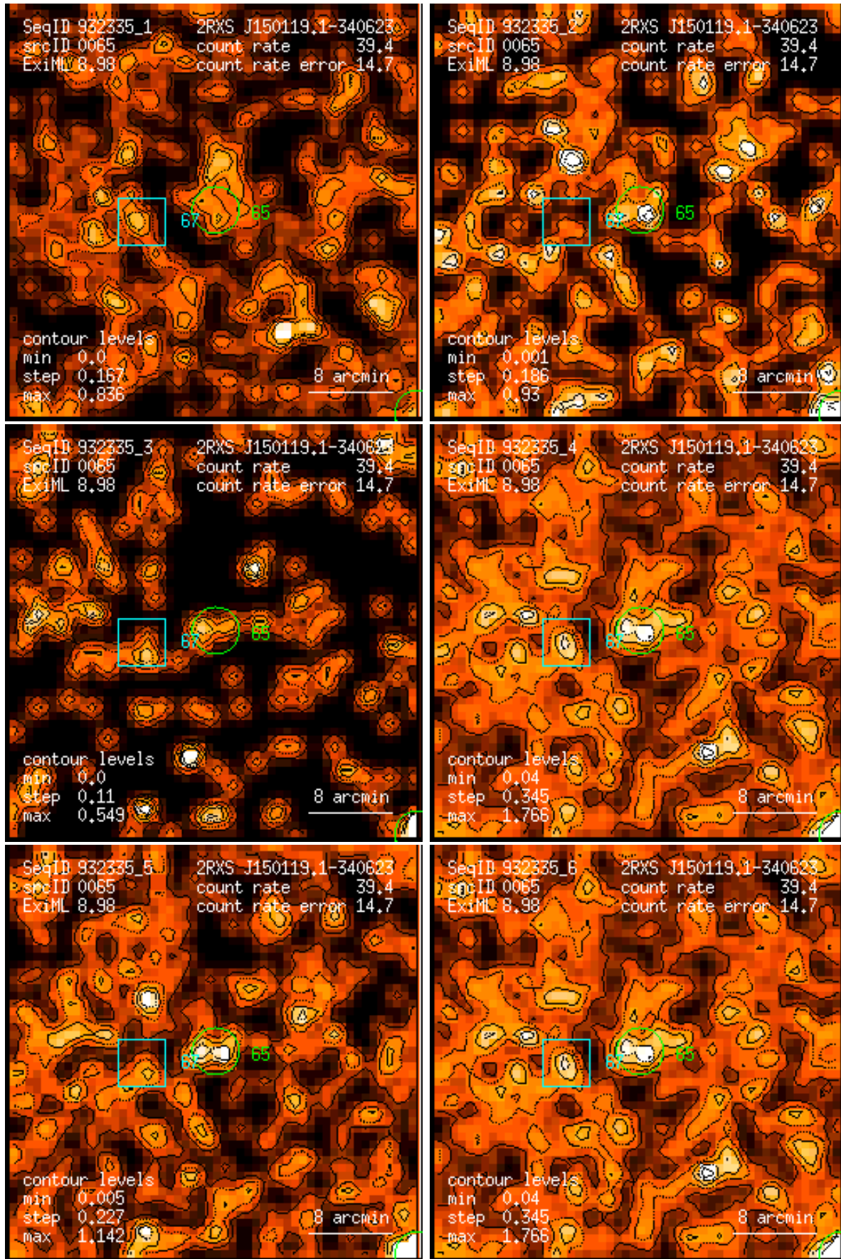
Figure 65: RASS 932335: detection 0065: band rate images, Gaussian filter: (1) PSPC channels 11 – 41, (2) 52 – 90, (3) 91 – 201, (4) 11 – 235, (5) 52 – 201, (6) 11 – 201. Broad band rates in counts/ks. Band rate contour levels in counts/ks/arcmin 2 .
