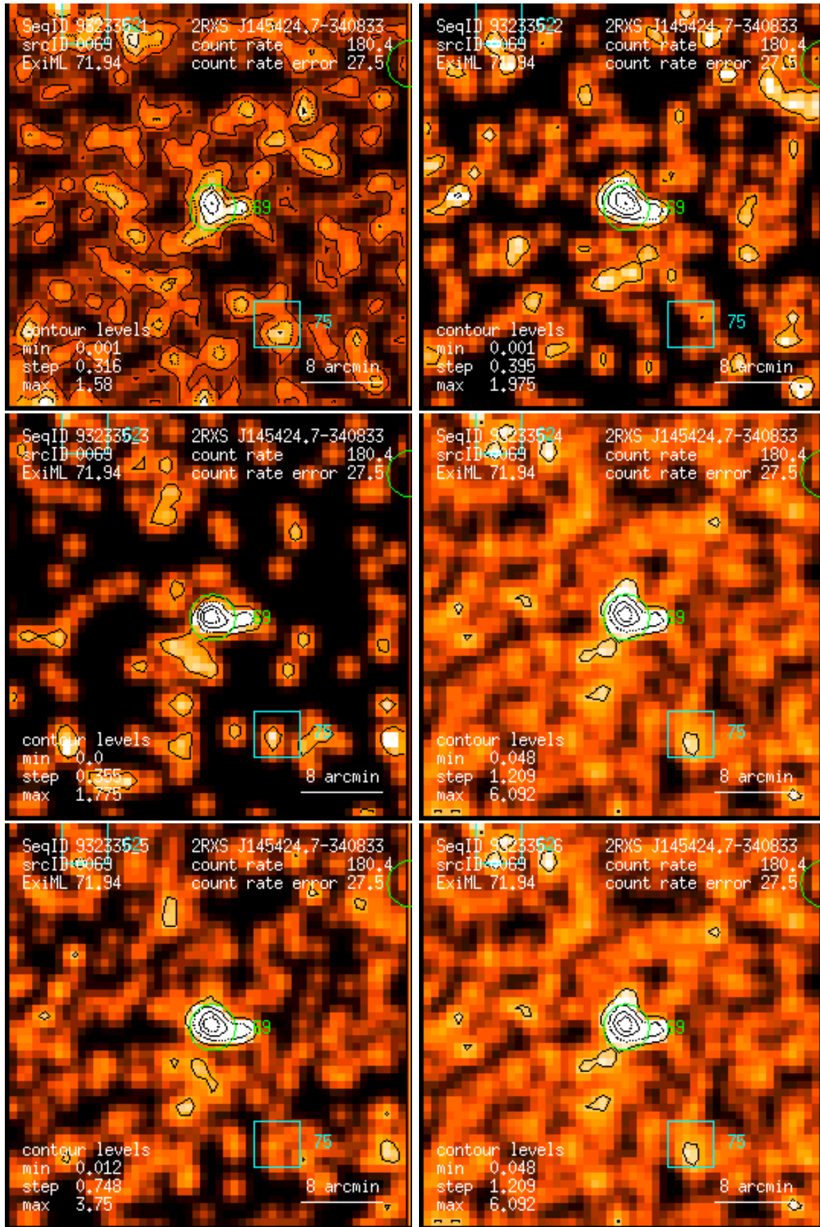
Figure 69: RASS 932335: detection 0069: band rate images, Gaussian filter: (1) PSPC channels 11 – 41, (2) 52 – 90, (3) 91 – 201, (4) 11 – 235, (5) 52 – 201, (6) 11 – 201. Broad band rates in counts/ks. Band rate contour levels in counts/ks/arcmin 2 .
