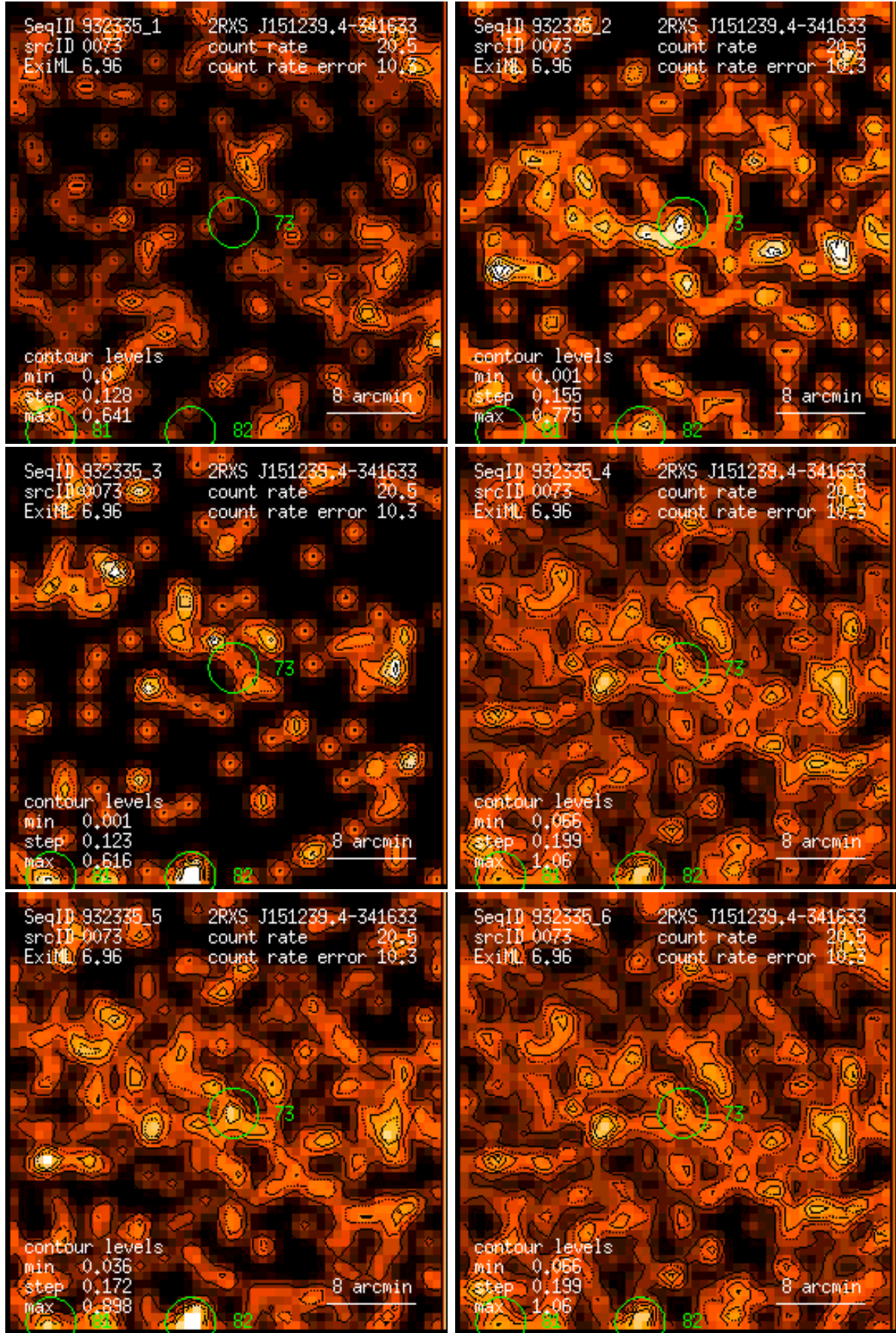
Figure 73: RASS 932335: detection 0073: band rate images, Gaussian filter: (1) PSPC channels 11 – 41, (2) 52 – 90, (3) 91 – 201, (4) 11 – 235, (5) 52 – 201, (6) 11 – 201. Broad band rates in counts/ks. Band rate contour levels in counts/ks/arcmin 2 .
