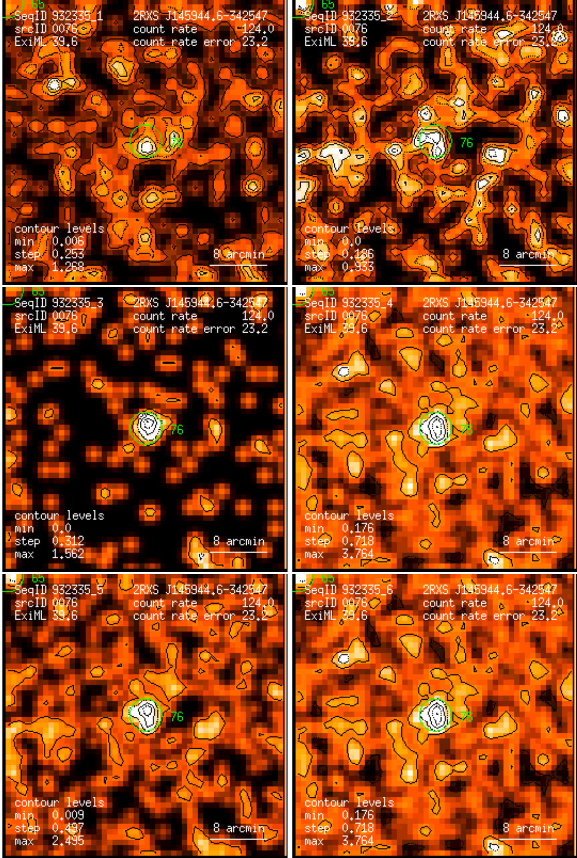
Figure 76: RASS 932335: detection 0076: band rate images, Gaussian filter: (1) PSPC channels 11 – 41, (2) 52 – 90, (3) 91 – 201, (4) 11 – 235, (5) 52 – 201, (6) 11 – 201. Broad band rates in counts/ks. Band rate contour levels in counts/ks/arcmin 2 .
