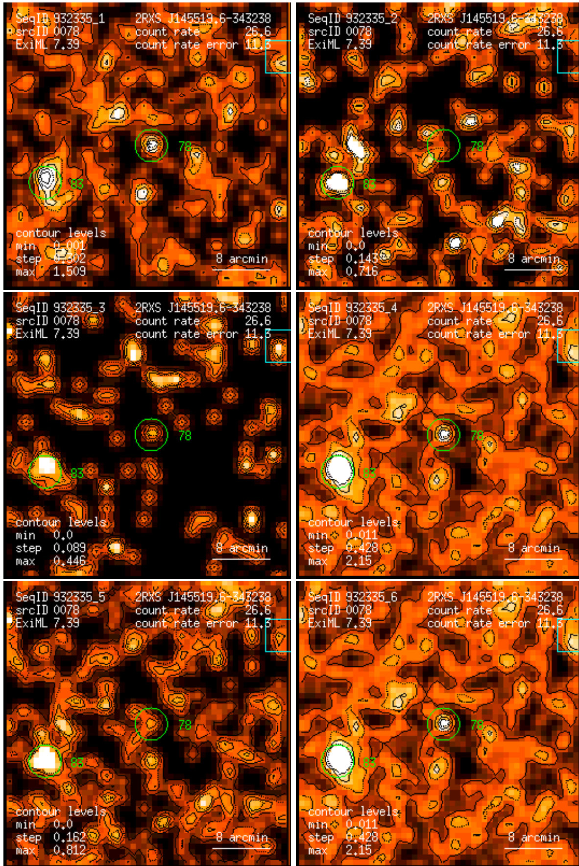
Figure 78: RASS 932335: detection 0078: band rate images, Gaussian filter: (1) PSPC channels 11 – 41, (2) 52 – 90, (3) 91 – 201, (4) 11 – 235, (5) 52 – 201, (6) 11 – 201. Broad band rates in counts/ks. Band rate contour levels in counts/ks/arcmin 2 .
