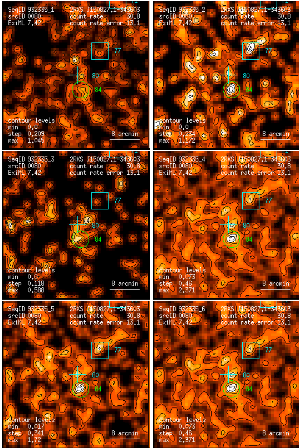
Figure 80: RASS 932335: detection 0080: band rate images, Gaussian filter: (1) PSPC channels 11 – 41, (2) 52 – 90, (3) 91 – 201, (4) 11 – 235, (5) 52 – 201, (6) 11 – 201. Broad band rates in counts/ks. Band rate contour levels in counts/ks/arcmin 2 .
