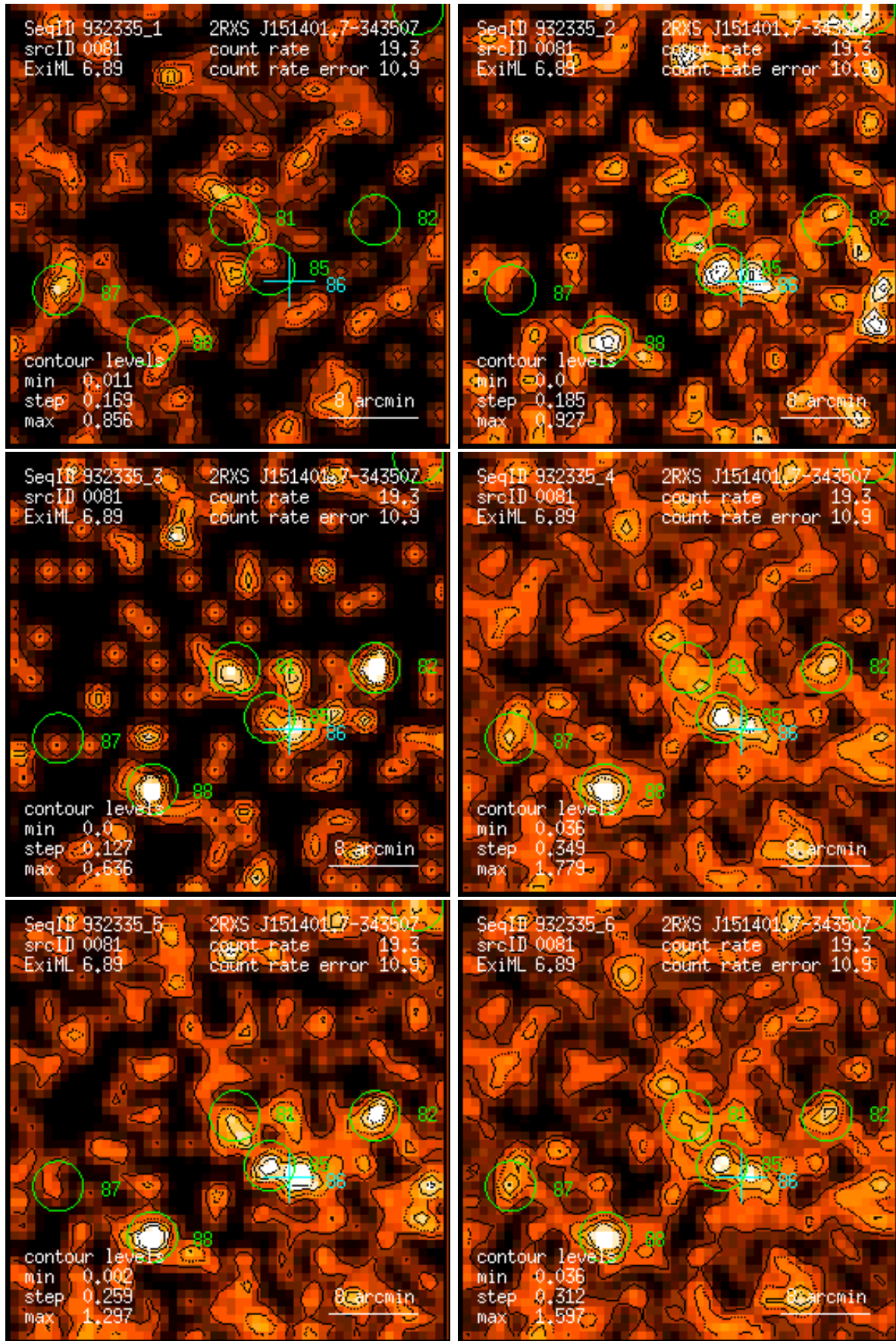
Figure 81: RASS 932335: detection 0081: band rate images, Gaussian filter: (1) PSPC channels 11 – 41, (2) 52 – 90, (3) 91 – 201, (4) 11 – 235, (5) 52 – 201, (6) 11 – 201. Broad band rates in counts/ks. Band rate contour levels in counts/ks/arcmin 2 .
