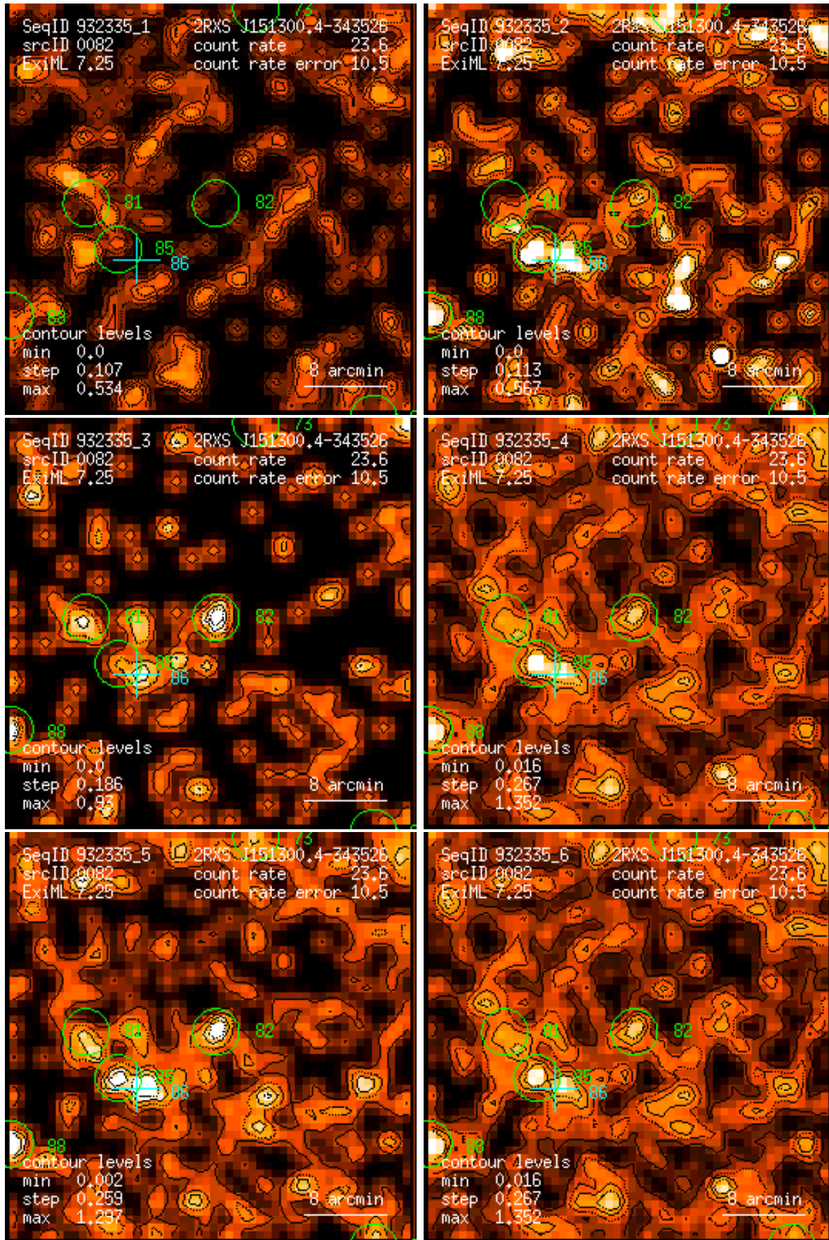
Figure 82: RASS 932335: detection 0082: band rate images, Gaussian filter: (1) PSPC channels 11 – 41, (2) 52 – 90, (3) 91 – 201, (4) 11 – 235, (5) 52 – 201, (6) 11 – 201. Broad band rates in counts/ks. Band rate contour levels in counts/ks/arcmin 2 .
