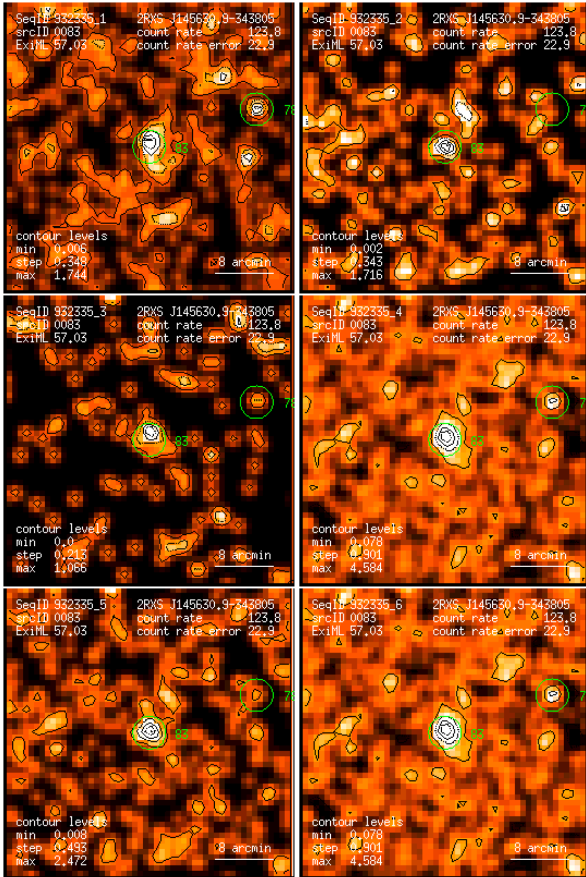
Figure 83: RASS 932335: detection 0083: band rate images, Gaussian filter: (1) PSPC channels 11 – 41, (2) 52 – 90, (3) 91 – 201, (4) 11 – 235, (5) 52 – 201, (6) 11 – 201. Broad band rates in counts/ks. Band rate contour levels in counts/ks/arcmin 2 .
