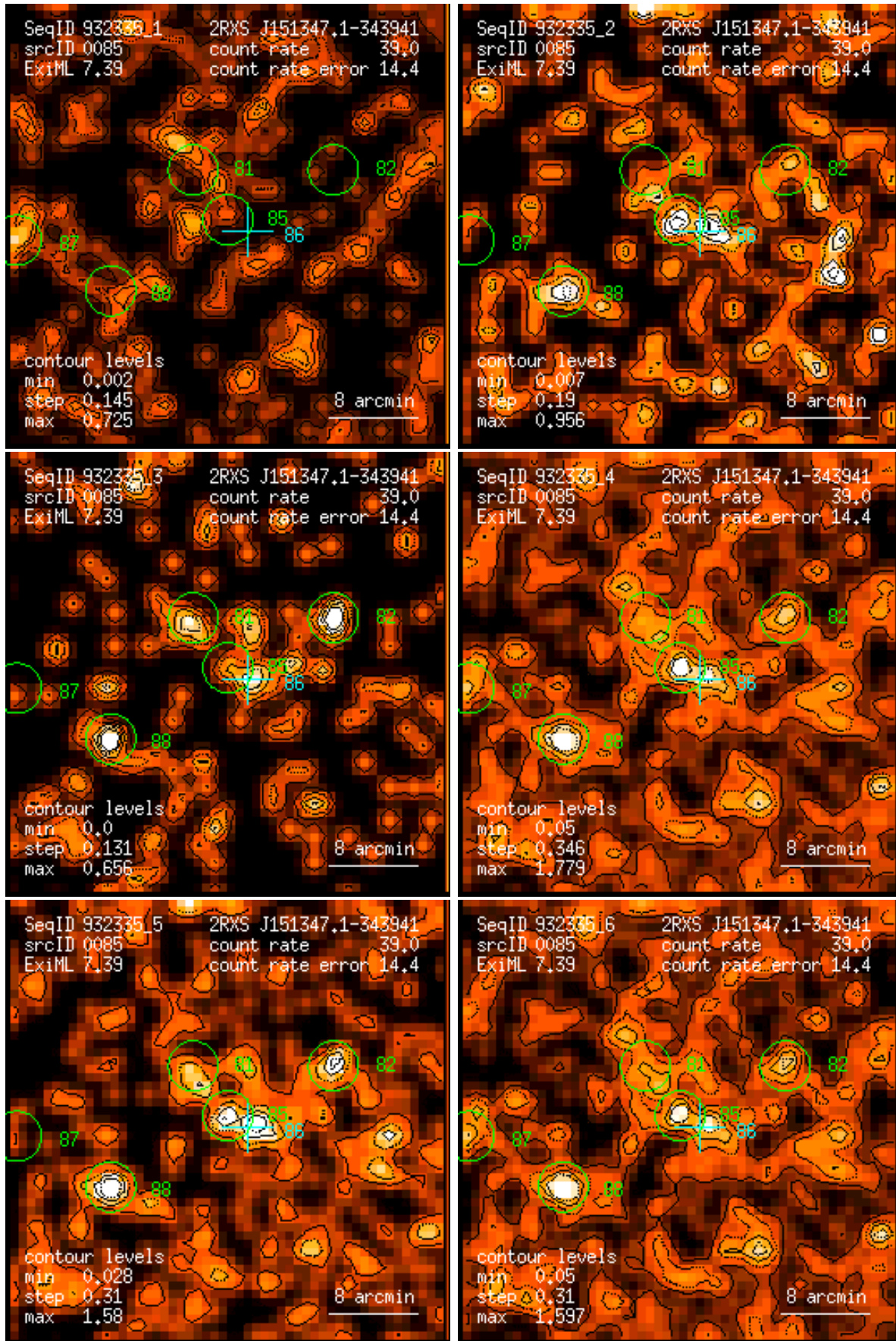
Figure 85: RASS 932335: detection 0085: band rate images, Gaussian filter: (1) PSPC channels 11 – 41, (2) 52 – 90, (3) 91 – 201, (4) 11 – 235, (5) 52 – 201, (6) 11 – 201. Broad band rates in counts/ks. Band rate contour levels in counts/ks/arcmin 2 .
