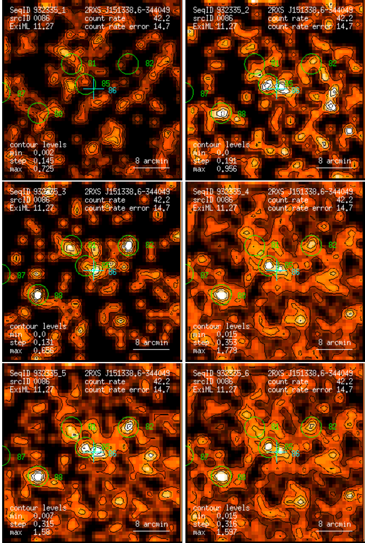
Figure 86: RASS 932335: detection 0086: band rate images, Gaussian filter: (1) PSPC channels 11 – 41, (2) 52 – 90, (3) 91 – 201, (4) 11 – 235, (5) 52 – 201, (6) 11 – 201. Broad band rates in counts/ks. Band rate contour levels in counts/ks/arcmin 2 .
