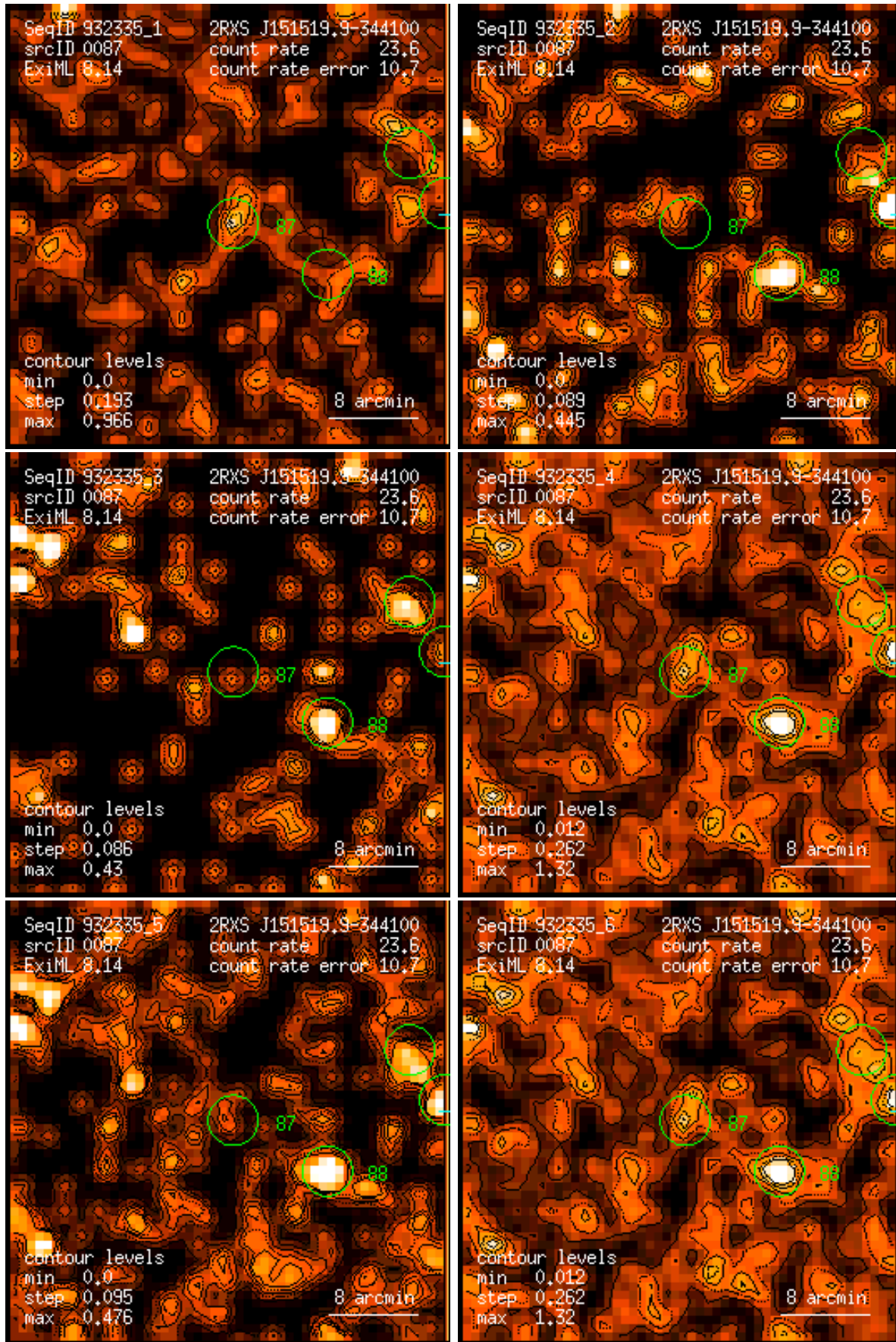
Figure 87: RASS 932335: detection 0087: band rate images, Gaussian filter: (1) PSPC channels 11 – 41, (2) 52 – 90, (3) 91 – 201, (4) 11 – 235, (5) 52 – 201, (6) 11 – 201. Broad band rates in counts/ks. Band rate contour levels in counts/ks/arcmin 2 .
