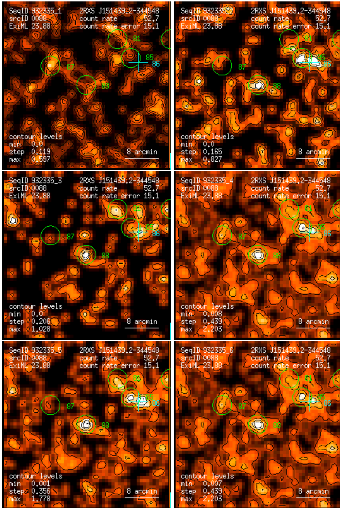
Figure 88: RASS 932335: detection 0088: band rate images, Gaussian filter: (1) PSPC channels 11 – 41, (2) 52 – 90, (3) 91 – 201, (4) 11 – 235, (5) 52 – 201, (6) 11 – 201. Broad band rates in counts/ks. Band rate contour levels in counts/ks/arcmin 2 .
