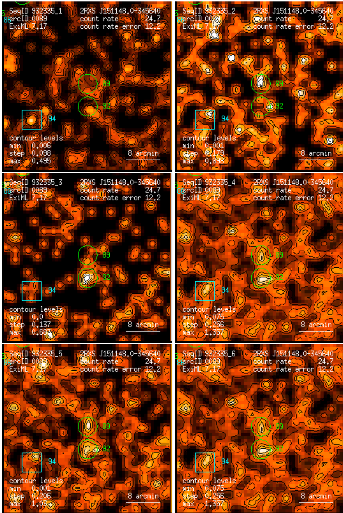
Figure 89: RASS 932335: detection 0089: band rate images, Gaussian filter: (1) PSPC channels 11 – 41, (2) 52 – 90, (3) 91 – 201, (4) 11 – 235, (5) 52 – 201, (6) 11 – 201. Broad band rates in counts/ks. Band rate contour levels in counts/ks/arcmin 2 .
