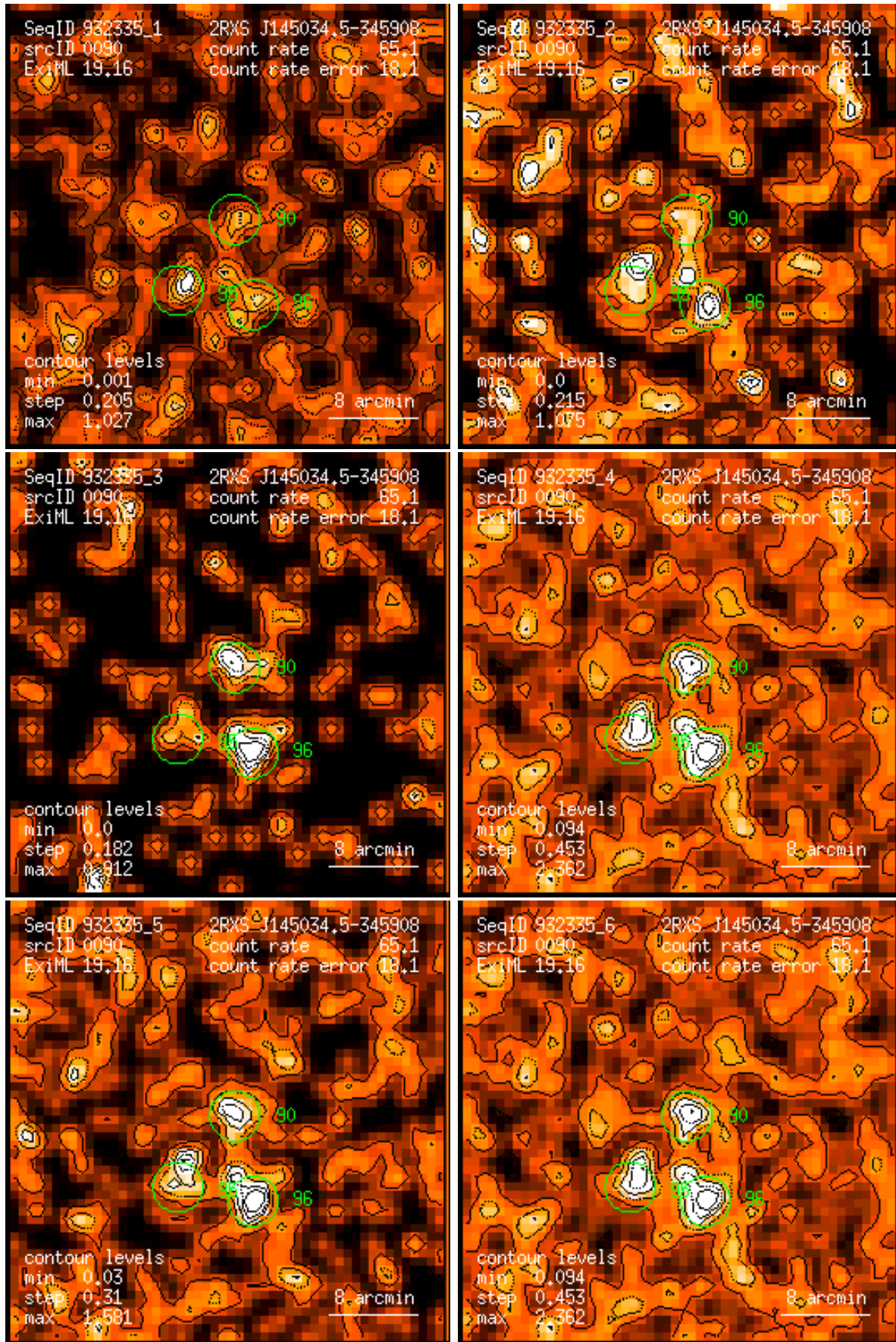
Figure 90: RASS 932335: detection 0090: band rate images, Gaussian filter: (1) PSPC channels 11 – 41, (2) 52 – 90, (3) 91 – 201, (4) 11 – 235, (5) 52 – 201, (6) 11 – 201. Broad band rates in counts/ks. Band rate contour levels in counts/ks/arcmin 2 .
