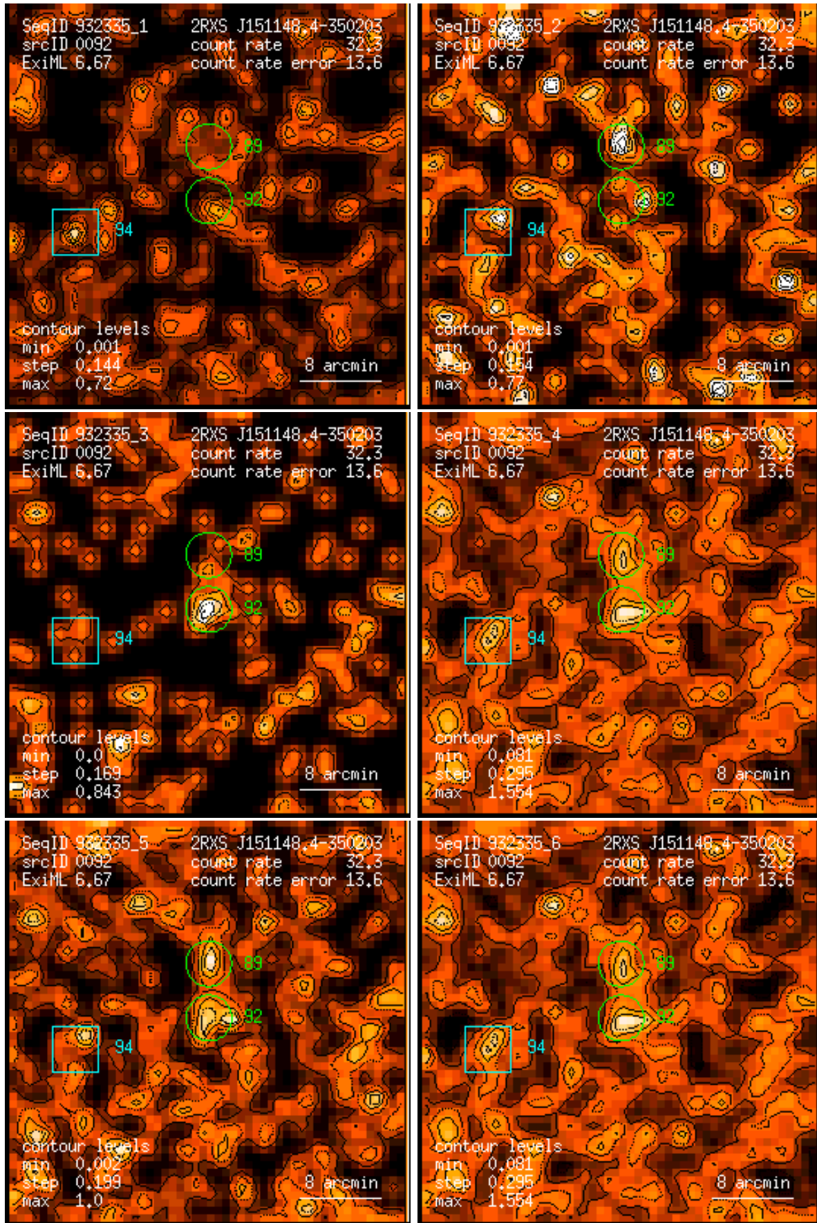
Figure 92: RASS 932335: detection 0092: band rate images, Gaussian filter: (1) PSPC channels 11 – 41, (2) 52 – 90, (3) 91 – 201, (4) 11 – 235, (5) 52 – 201, (6) 11 – 201. Broad band rates in counts/ks. Band rate contour levels in counts/ks/arcmin 2 .
