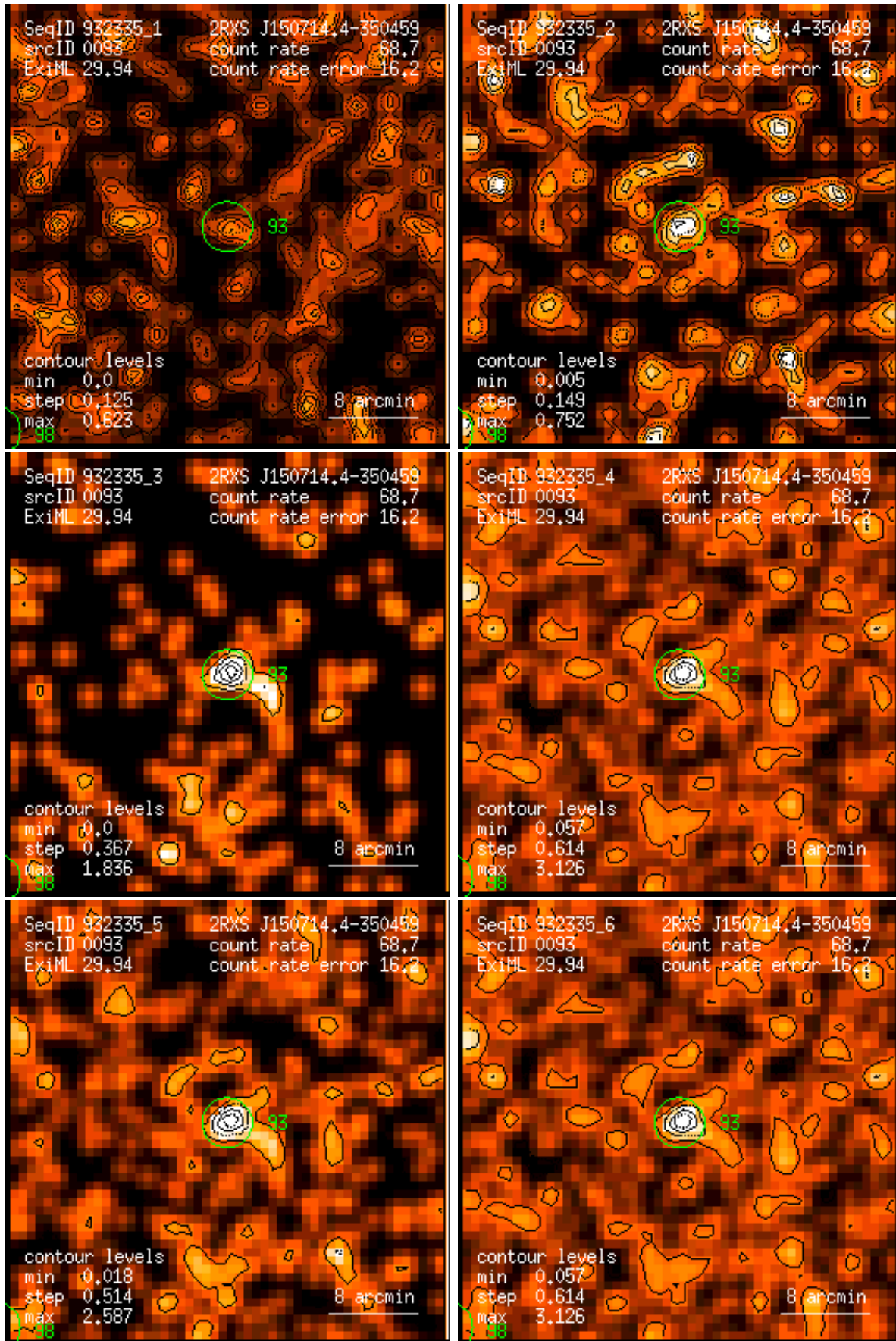
Figure 93: RASS 932335: detection 0093: band rate images, Gaussian filter: (1) PSPC channels 11 – 41, (2) 52 – 90, (3) 91 – 201, (4) 11 – 235, (5) 52 – 201, (6) 11 – 201. Broad band rates in counts/ks. Band rate contour levels in counts/ks/arcmin 2 .
