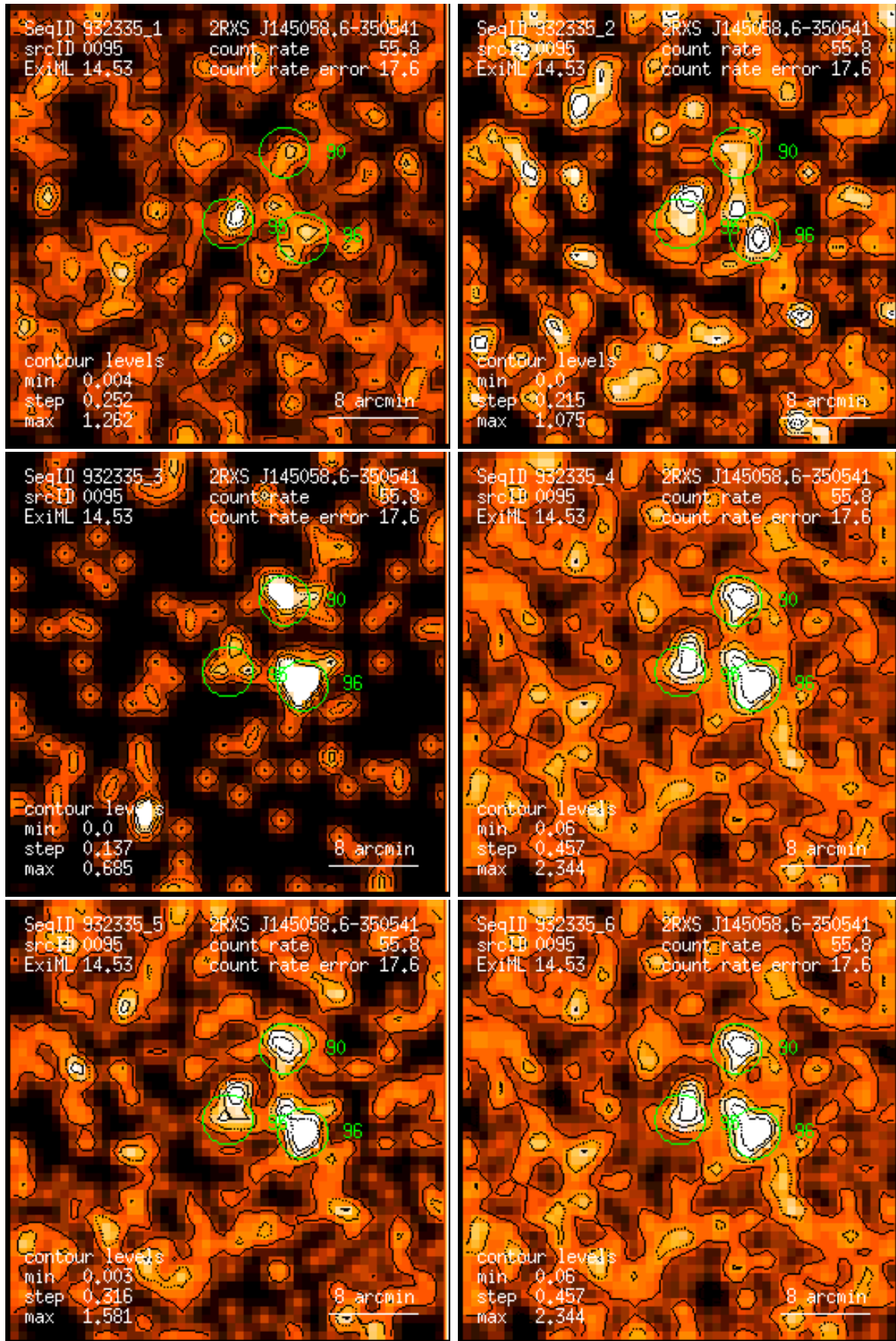
Figure 95: RASS 932335: detection 0095: band rate images, Gaussian filter: (1) PSPC channels 11 – 41, (2) 52 – 90, (3) 91 – 201, (4) 11 – 235, (5) 52 – 201, (6) 11 – 201. Broad band rates in counts/ks. Band rate contour levels in counts/ks/arcmin 2 .
