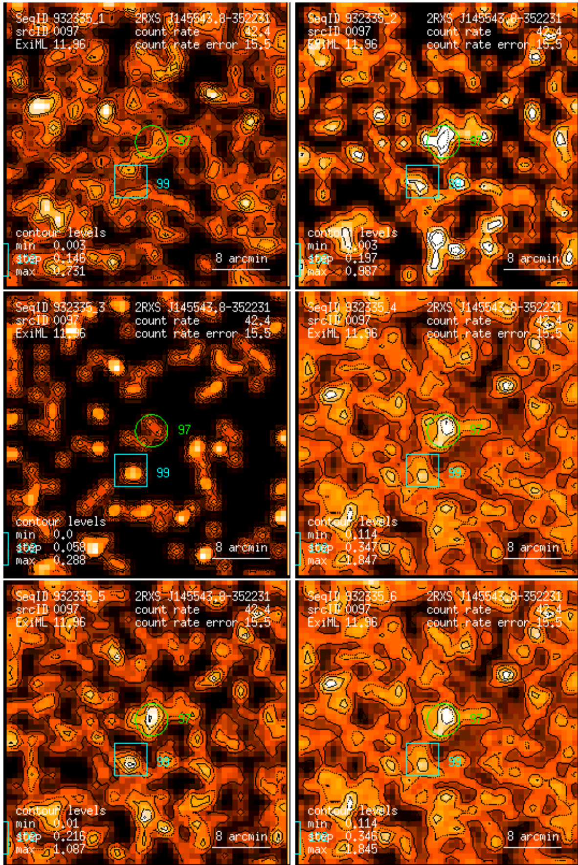
Figure 97: RASS 932335: detection 0097: band rate images, Gaussian filter: (1) PSPC channels 11 – 41, (2) 52 – 90, (3) 91 – 201, (4) 11 – 235, (5) 52 – 201, (6) 11 – 201. Broad band rates in counts/ks. Band rate contour levels in counts/ks/arcmin 2 .
