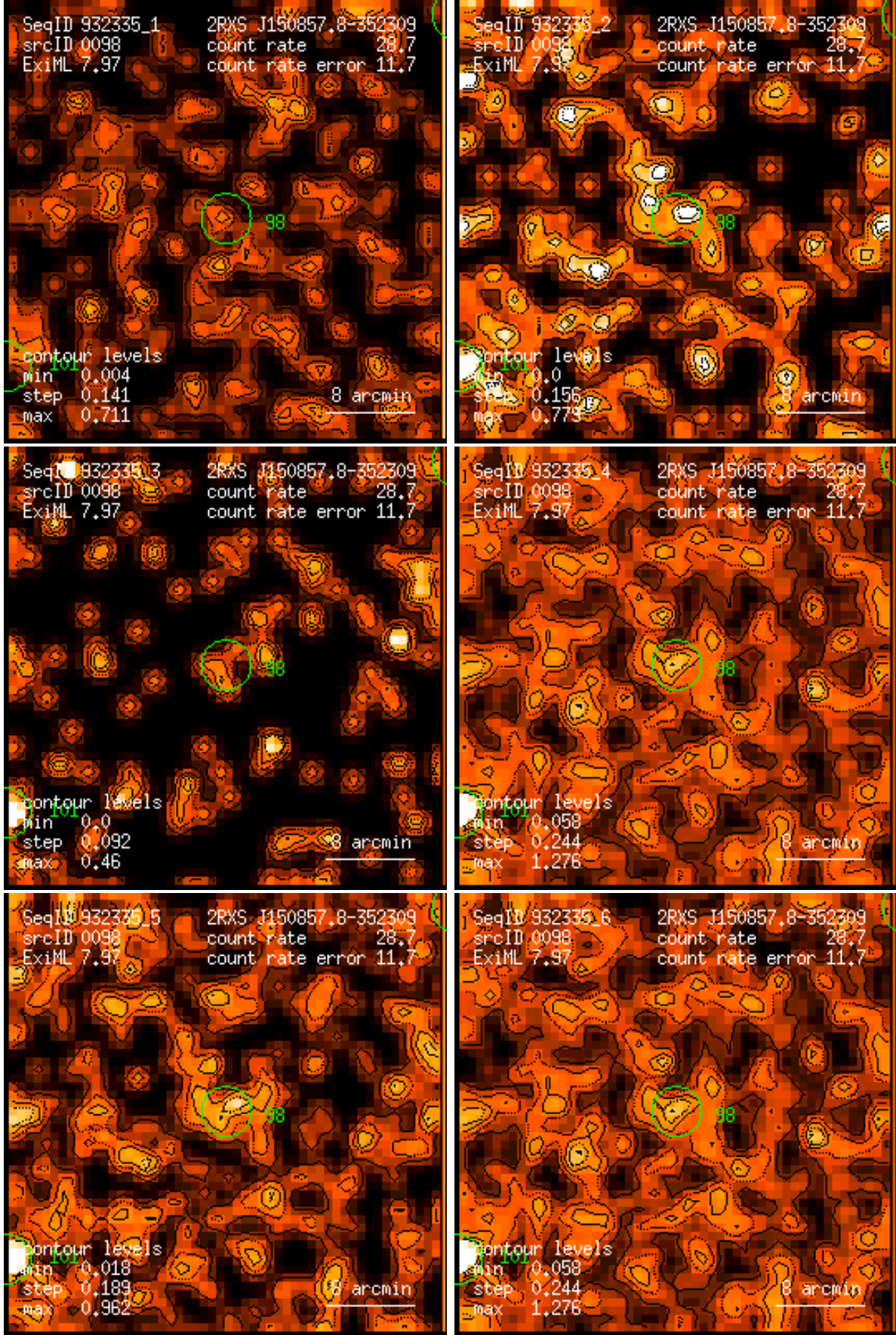
Figure 98: RASS 932335: detection 0098: band rate images, Gaussian filter: (1) PSPC channels 11 – 41, (2) 52 – 90, (3) 91 – 201, (4) 11 – 235, (5) 52 – 201, (6) 11 – 201. Broad band rates in counts/ks. Band rate contour levels in counts/ks/arcmin 2 .
