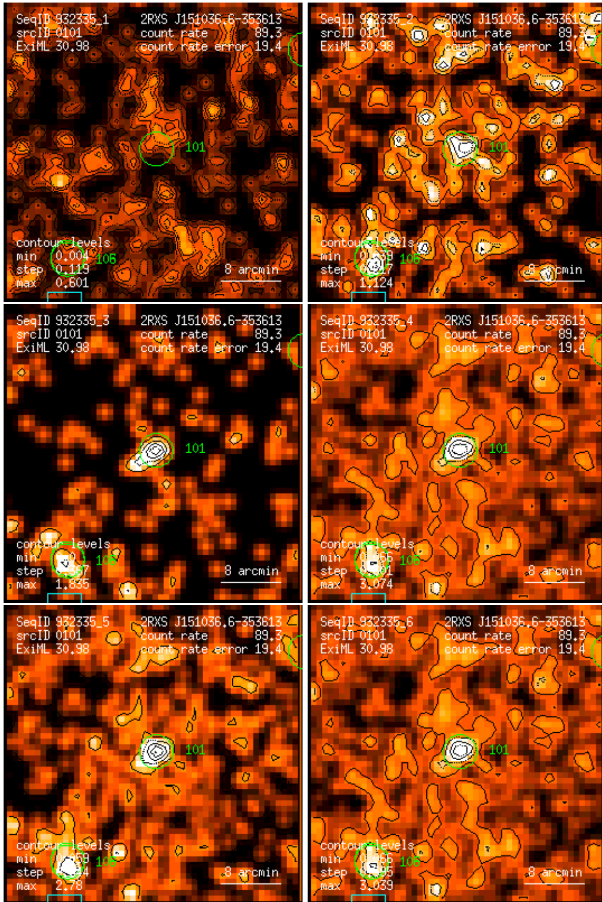
Figure 101: RASS 932335: detection 0101: band rate images, Gaussian filter: (1) PSPC channels 11 – 41, (2) 52 – 90, (3) 91 – 201, (4) 11 – 235, (5) 52 – 201, (6) 11 – 201. Broad band rates in counts/ks. Band rate contour levels in counts/ks/arcmin 2 .
