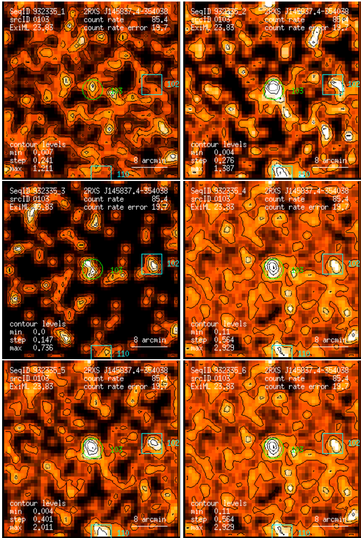
Figure 103: RASS 932335: detection 0103: band rate images, Gaussian filter: (1) PSPC channels 11 – 41, (2) 52 – 90, (3) 91 – 201, (4) 11 – 235, (5) 52 – 201, (6) 11 – 201. Broad band rates in counts/ks. Band rate contour levels in counts/ks/arcmin 2 .
