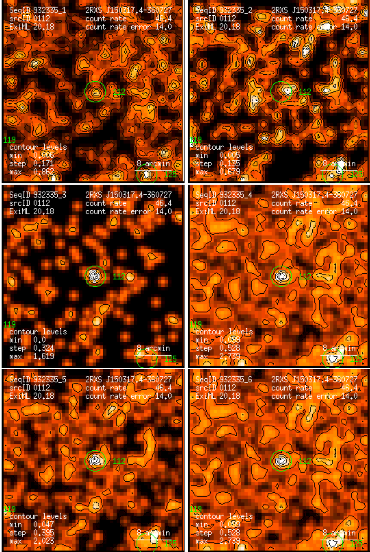
Figure 112: RASS 932335: detection 0112: band rate images, Gaussian filter: (1) PSPC channels 11 – 41, (2) 52 – 90, (3) 91 – 201, (4) 11 – 235, (5) 52 – 201, (6) 11 – 201. Broad band rates in counts/ks. Band rate contour levels in counts/ks/arcmin 2 .
