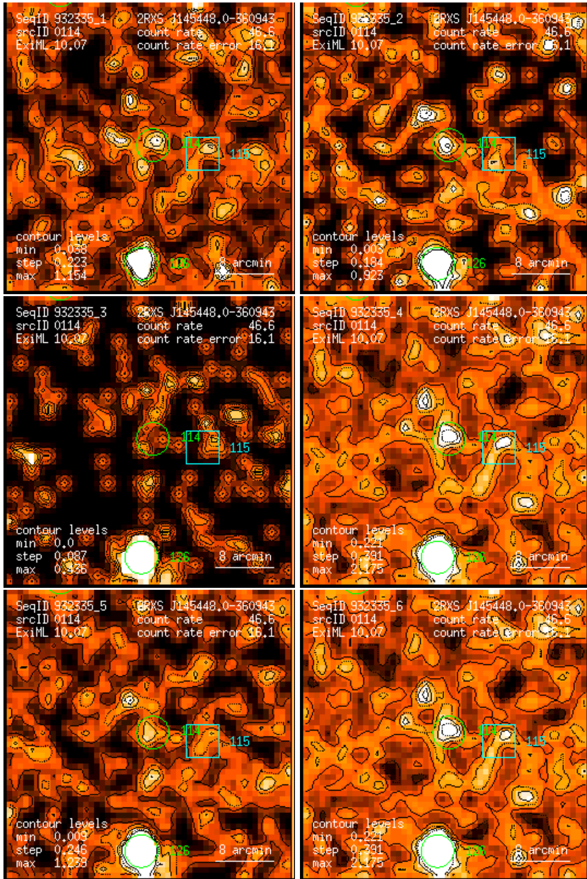
Figure 114: RASS 932335: detection 0114: band rate images, Gaussian filter: (1) PSPC channels 11 – 41, (2) 52 – 90, (3) 91 – 201, (4) 11 – 235, (5) 52 – 201, (6) 11 – 201. Broad band rates in counts/ks. Band rate contour levels in counts/ks/arcmin 2 .
