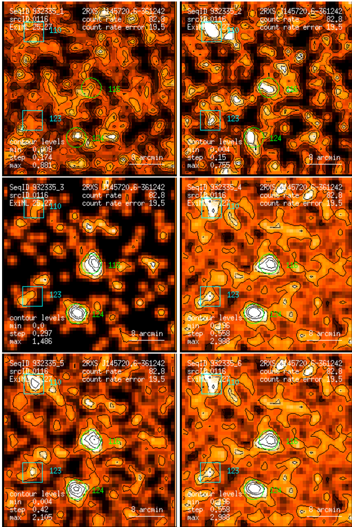
Figure 116: RASS 932335: detection 0116: band rate images, Gaussian filter: (1) PSPC channels 11 – 41, (2) 52 – 90, (3) 91 – 201, (4) 11 – 235, (5) 52 – 201, (6) 11 – 201. Broad band rates in counts/ks. Band rate contour levels in counts/ks/arcmin 2 .
