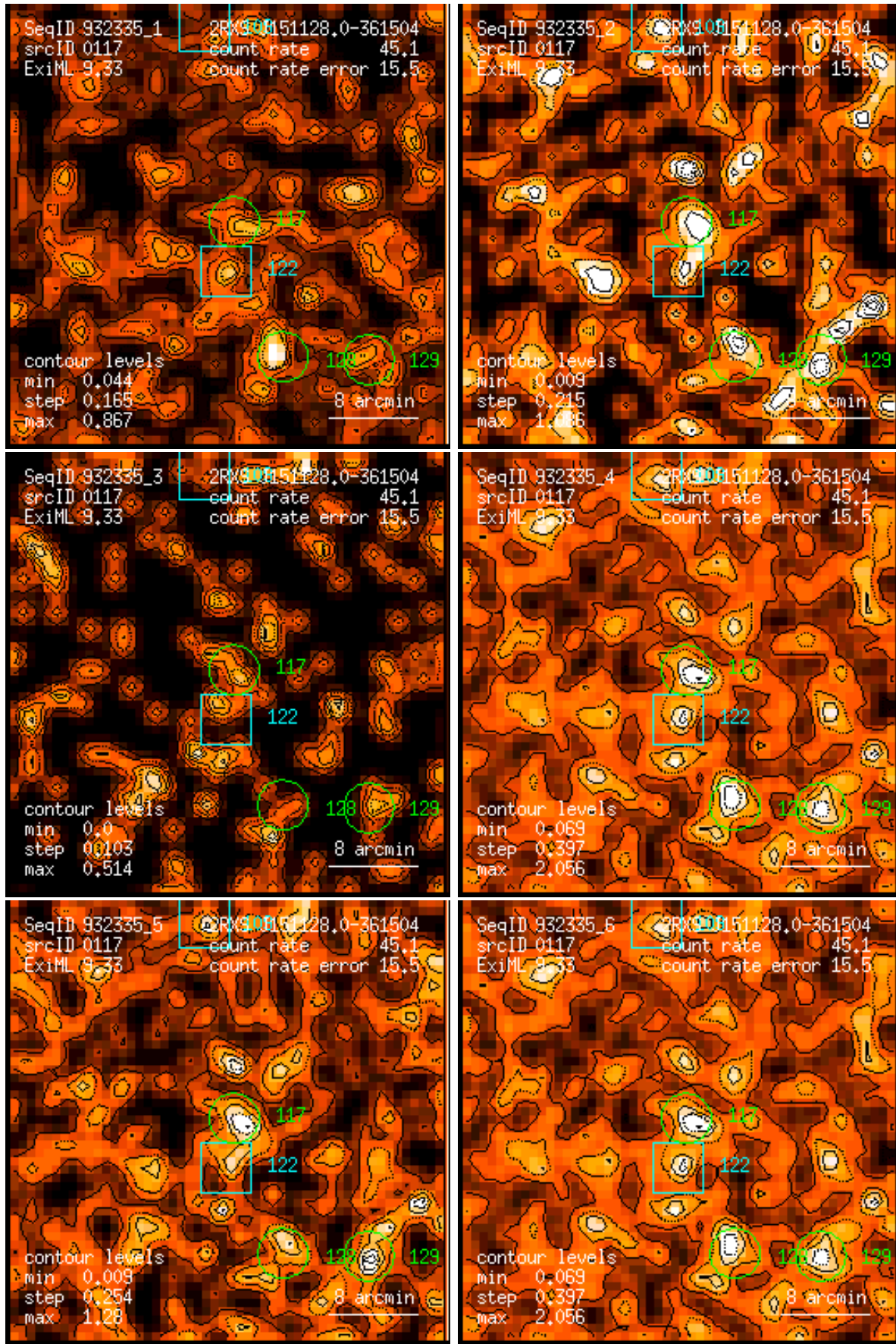
Figure 117: RASS 932335: detection 0117: band rate images, Gaussian filter: (1) PSPC channels 11 – 41, (2) 52 – 90, (3) 91 – 201, (4) 11 – 235, (5) 52 – 201, (6) 11 – 201. Broad band rates in counts/ks. Band rate contour levels in counts/ks/arcmin 2 .
