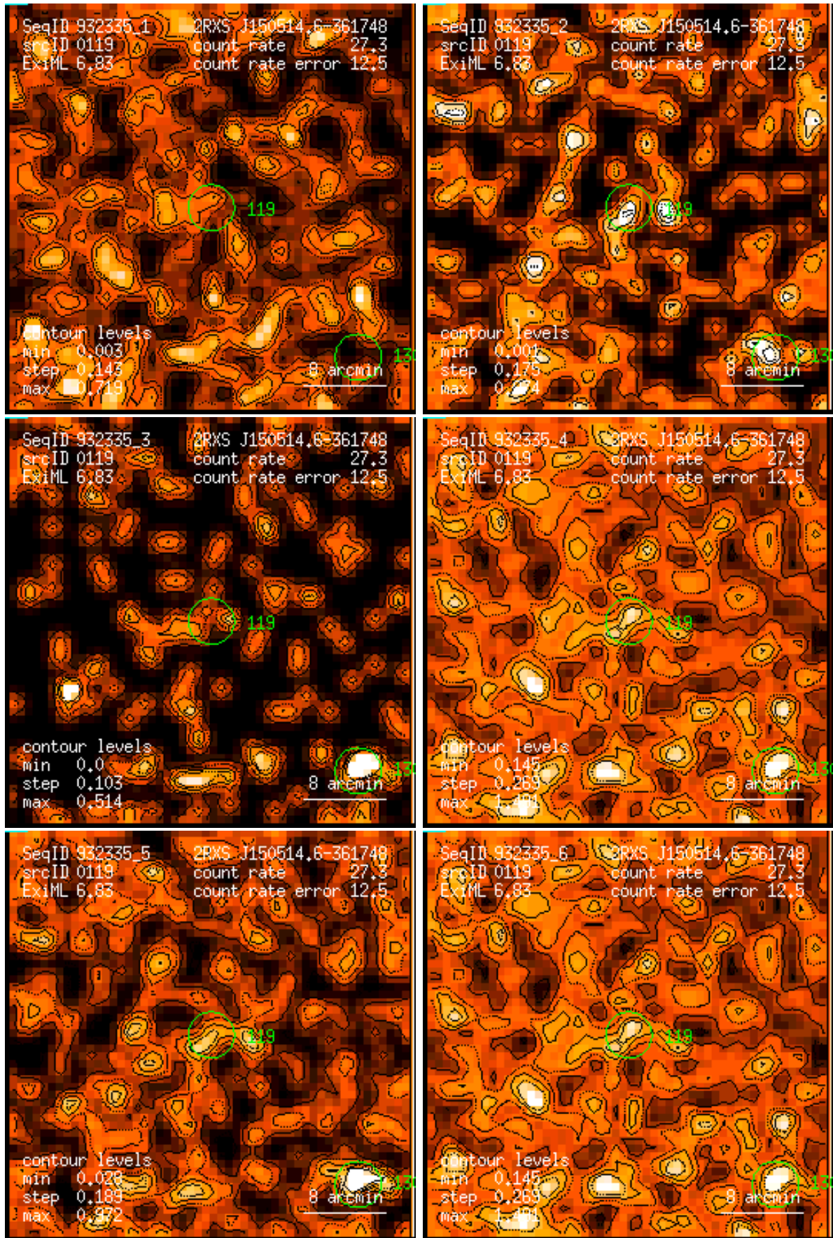
Figure 119: RASS 932335: detection 0119: band rate images, Gaussian filter: (1) PSPC channels 11 – 41, (2) 52 – 90, (3) 91 – 201, (4) 11 – 235, (5) 52 – 201, (6) 11 – 201. Broad band rates in counts/ks. Band rate contour levels in counts/ks/arcmin 2 .
