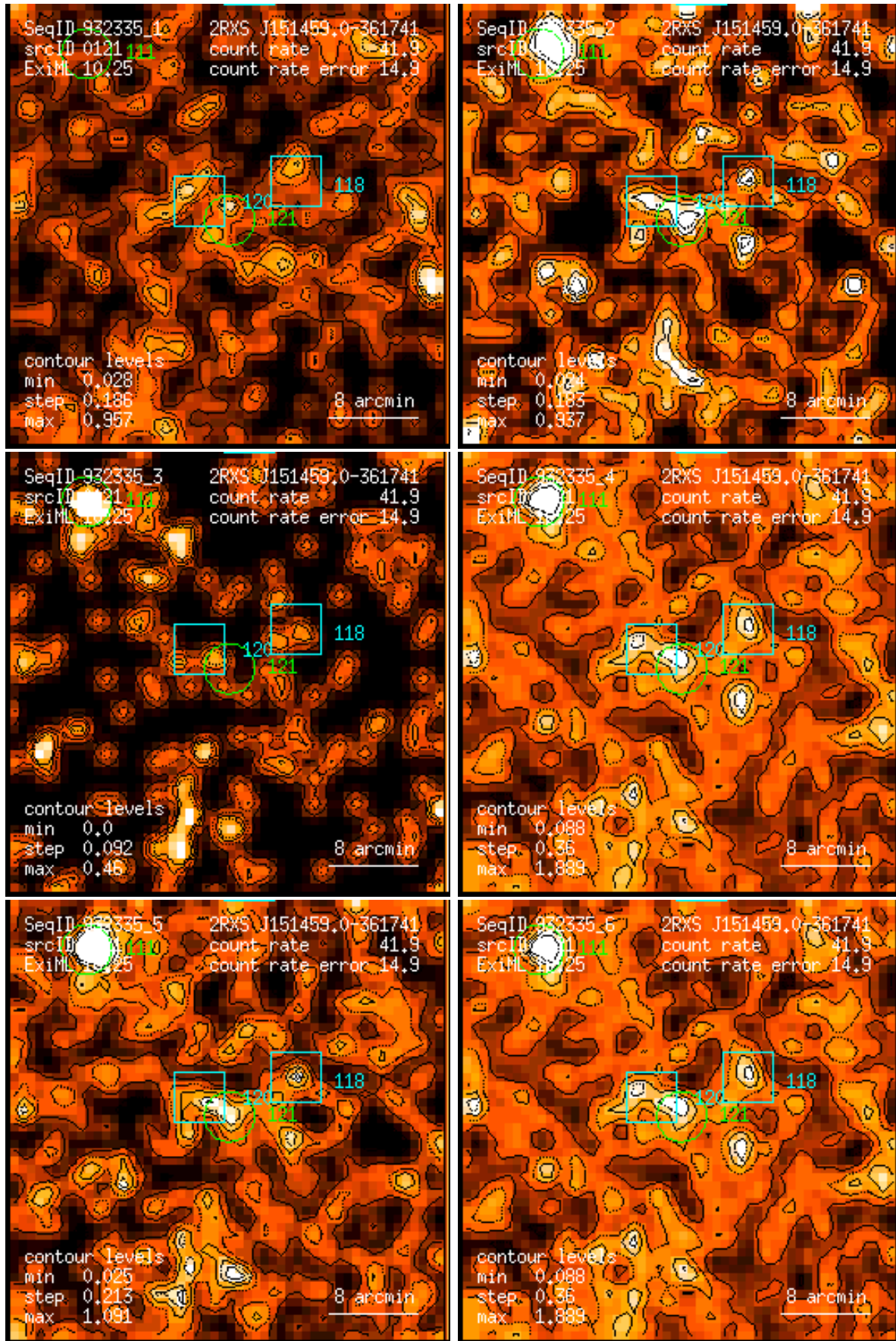
Figure 121: RASS 932335: detection 0121: band rate images, Gaussian filter: (1) PSPC channels 11 – 41, (2) 52 – 90, (3) 91 – 201, (4) 11 – 235, (5) 52 – 201, (6) 11 – 201. Broad band rates in counts/ks. Band rate contour levels in counts/ks/arcmin 2 .
