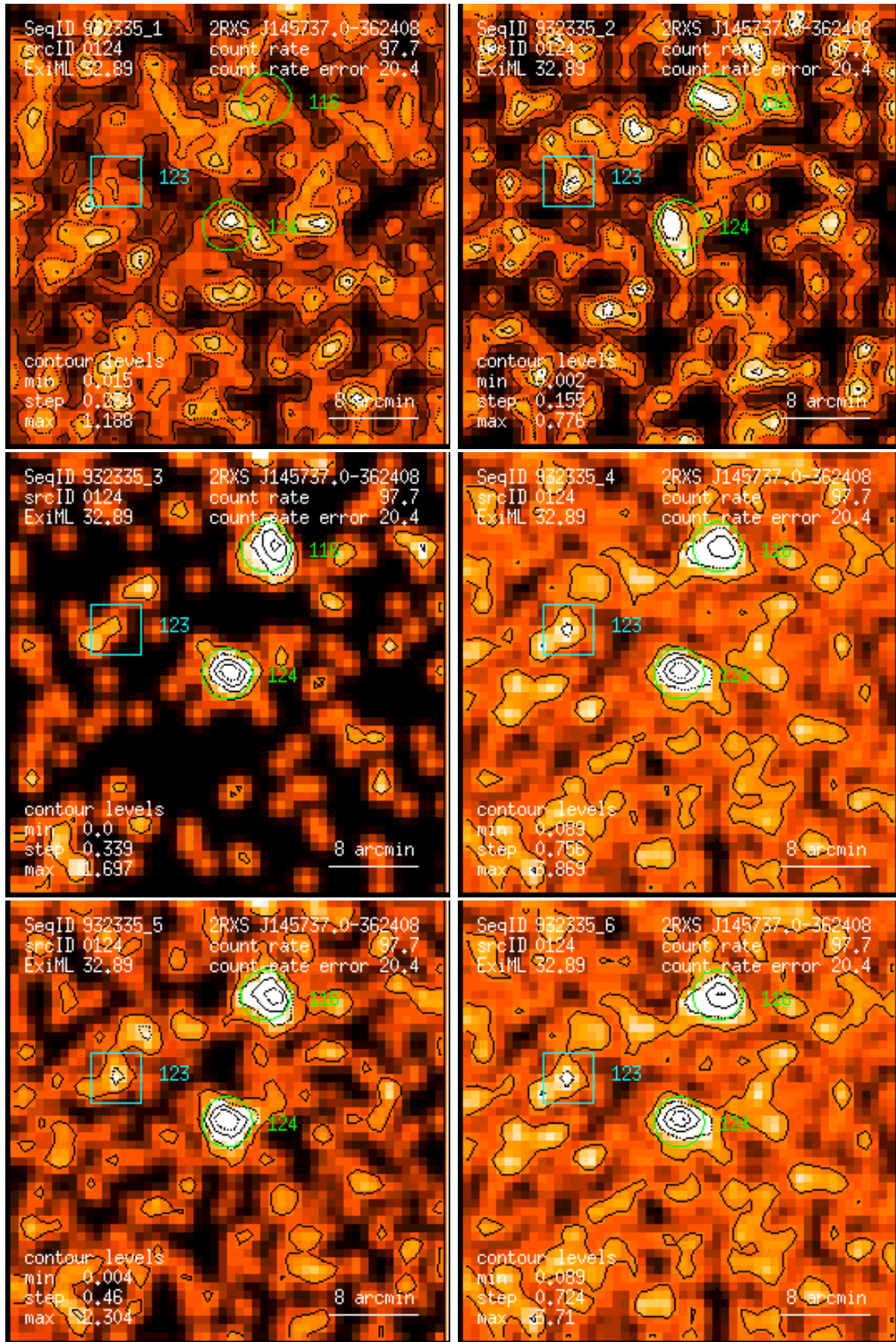
Figure 124: RASS 932335: detection 0124: band rate images, Gaussian filter: (1) PSPC channels 11 – 41, (2) 52 – 90, (3) 91 – 201, (4) 11 – 235, (5) 52 – 201, (6) 11 – 201. Broad band rates in counts/ks. Band rate contour levels in counts/ks/arcmin 2 .
