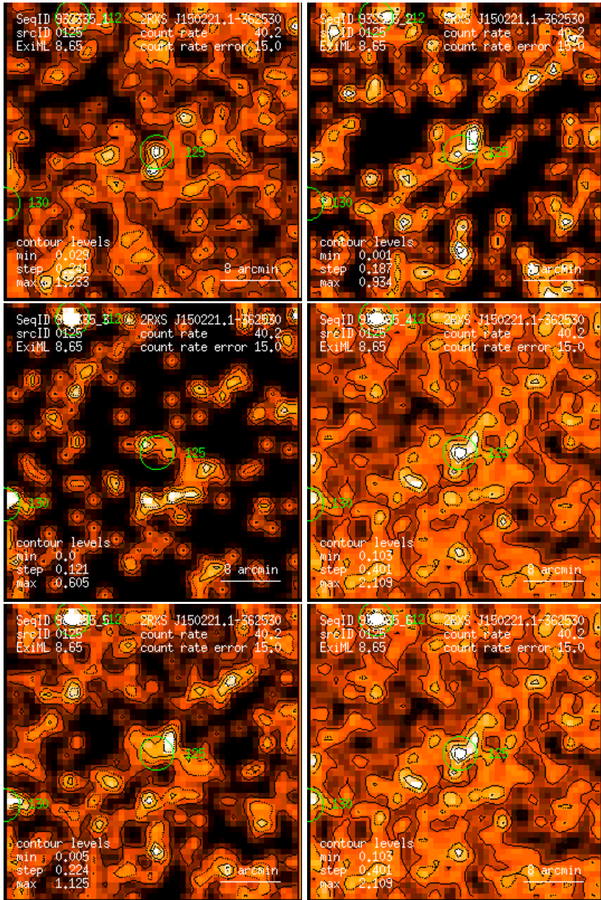
Figure 125: RASS 932335: detection 0125: band rate images, Gaussian filter: (1) PSPC channels 11 – 41, (2) 52 – 90, (3) 91 – 201, (4) 11 – 235, (5) 52 – 201, (6) 11 – 201. Broad band rates in counts/ks. Band rate contour levels in counts/ks/arcmin 2 .
