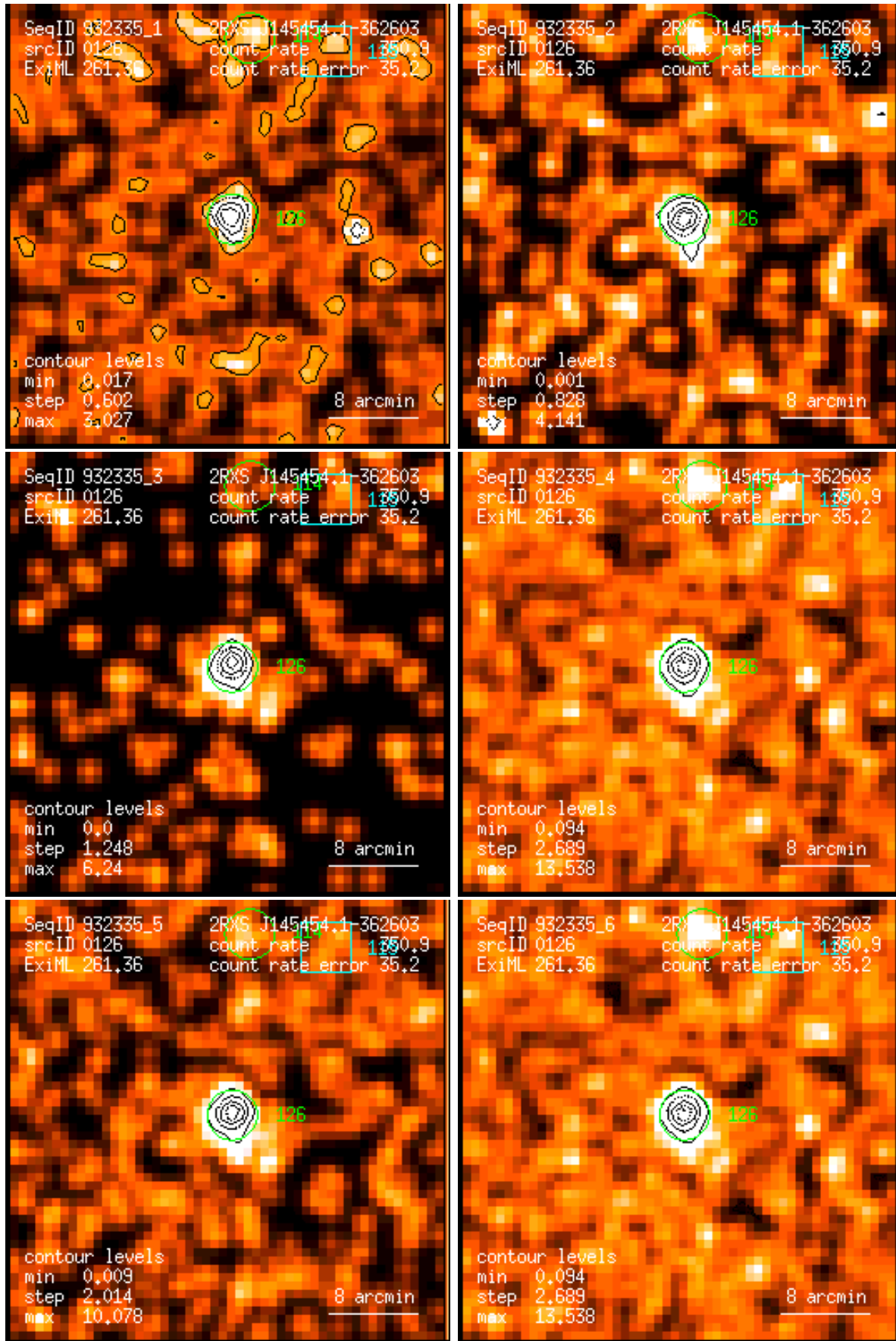
Figure 126: RASS 932335: detection 0126: band rate images, Gaussian filter: (1) PSPC channels 11 – 41, (2) 52 – 90, (3) 91 – 201, (4) 11 – 235, (5) 52 – 201, (6) 11 – 201. Broad band rates in counts/ks. Band rate contour levels in counts/ks/arcmin 2 .
