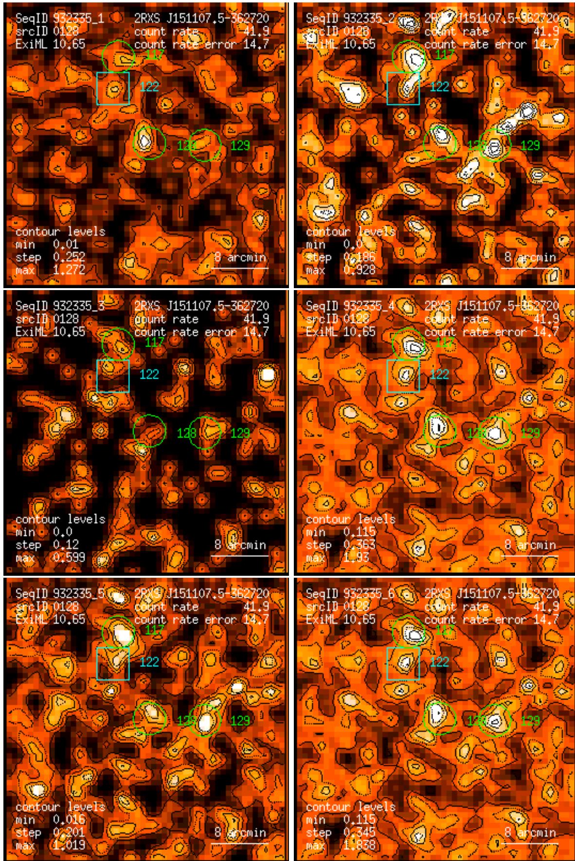
Figure 128: RASS 932335: detection 0128: band rate images, Gaussian filter: (1) PSPC channels 11 – 41, (2) 52 – 90, (3) 91 – 201, (4) 11 – 235, (5) 52 – 201, (6) 11 – 201. Broad band rates in counts/ks. Band rate contour levels in counts/ks/arcmin 2 .
